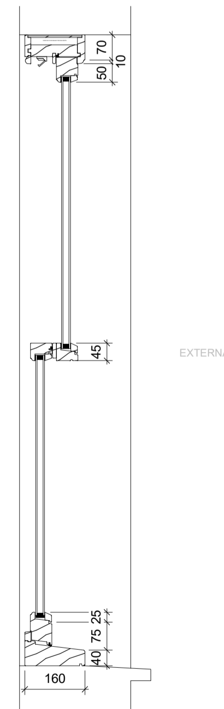
SECTION B-B
