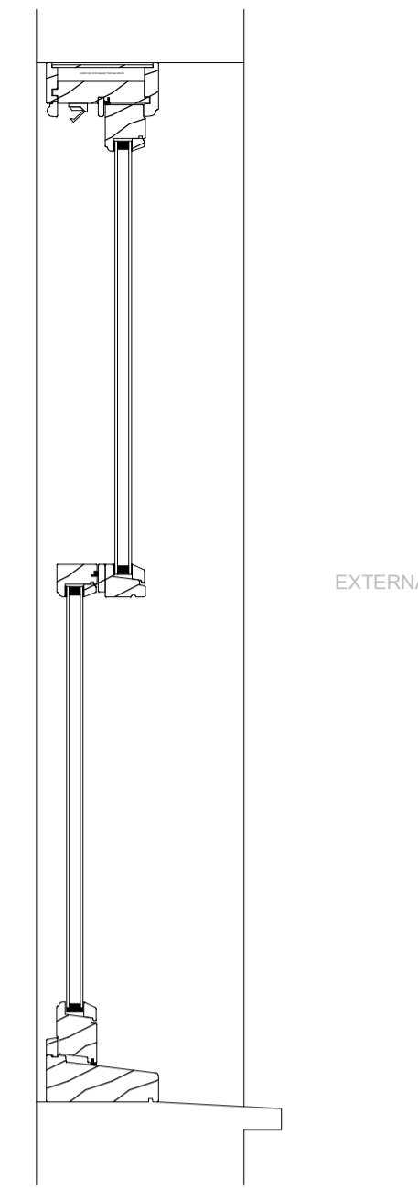
SECTION B-B
