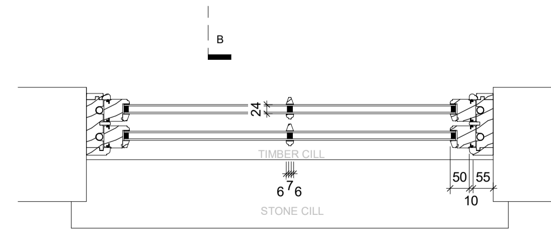
LOWER WINDOW DETAILS
