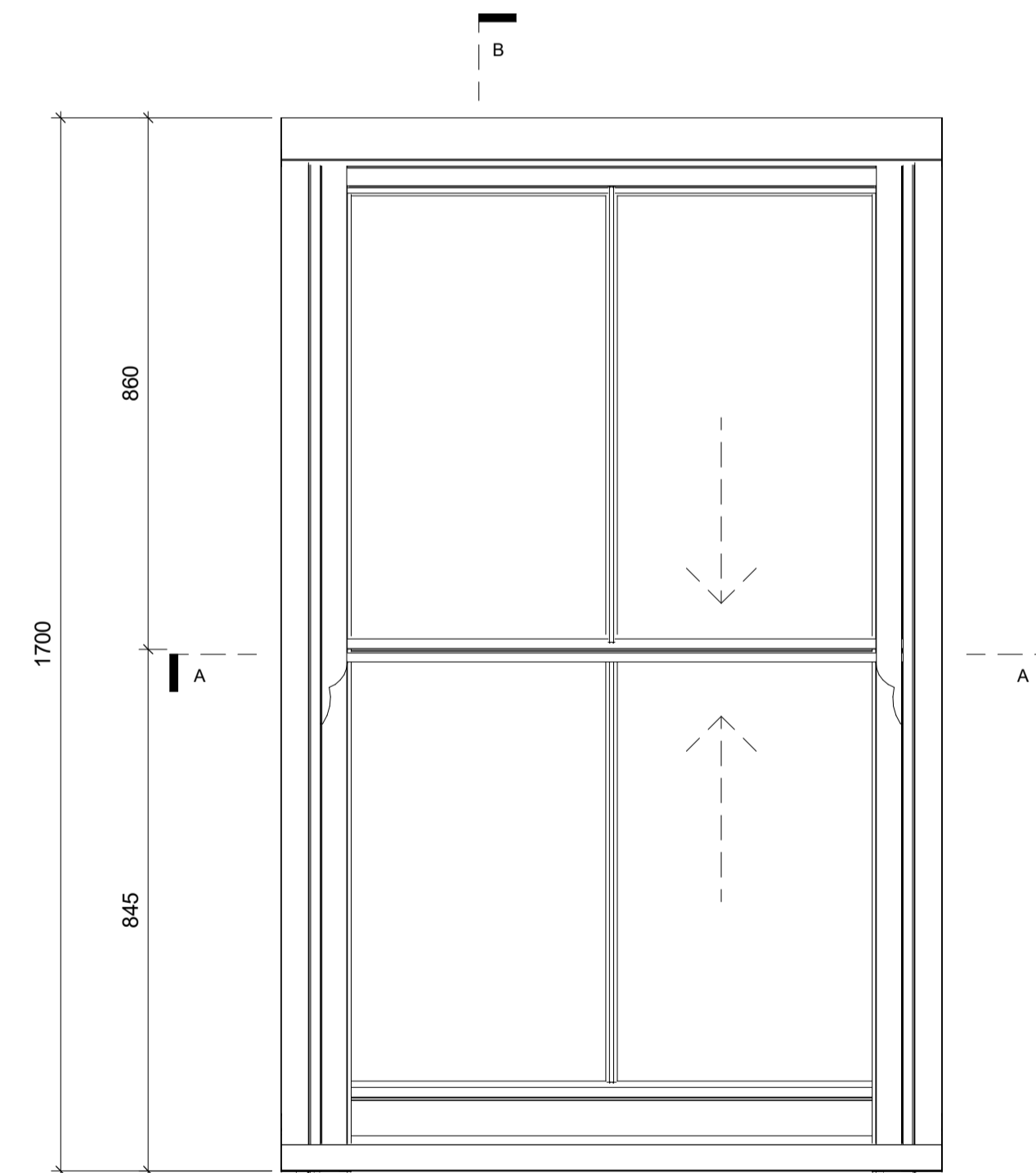
UPPER WINDOW DETAILS
