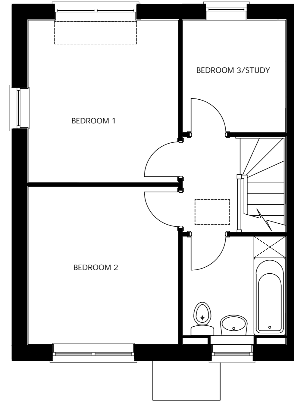
House Type A FIRST FLOOR PLAN
