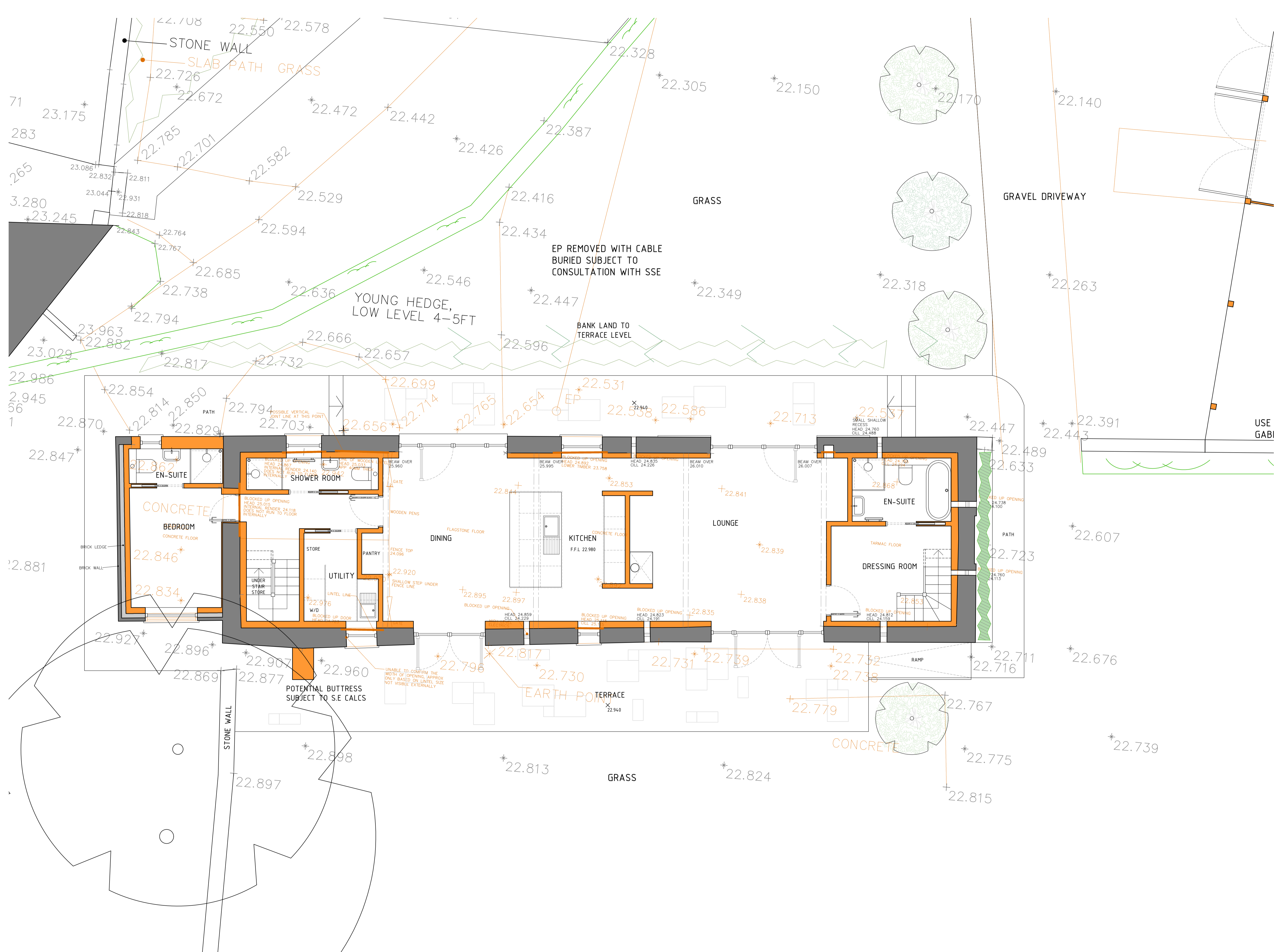
PROPOSED GROUND FLOOR DEMOLITION PLAN 1:100 @ A3 // 1:50 @ A1 0 1 2 3 4 5 METRES
