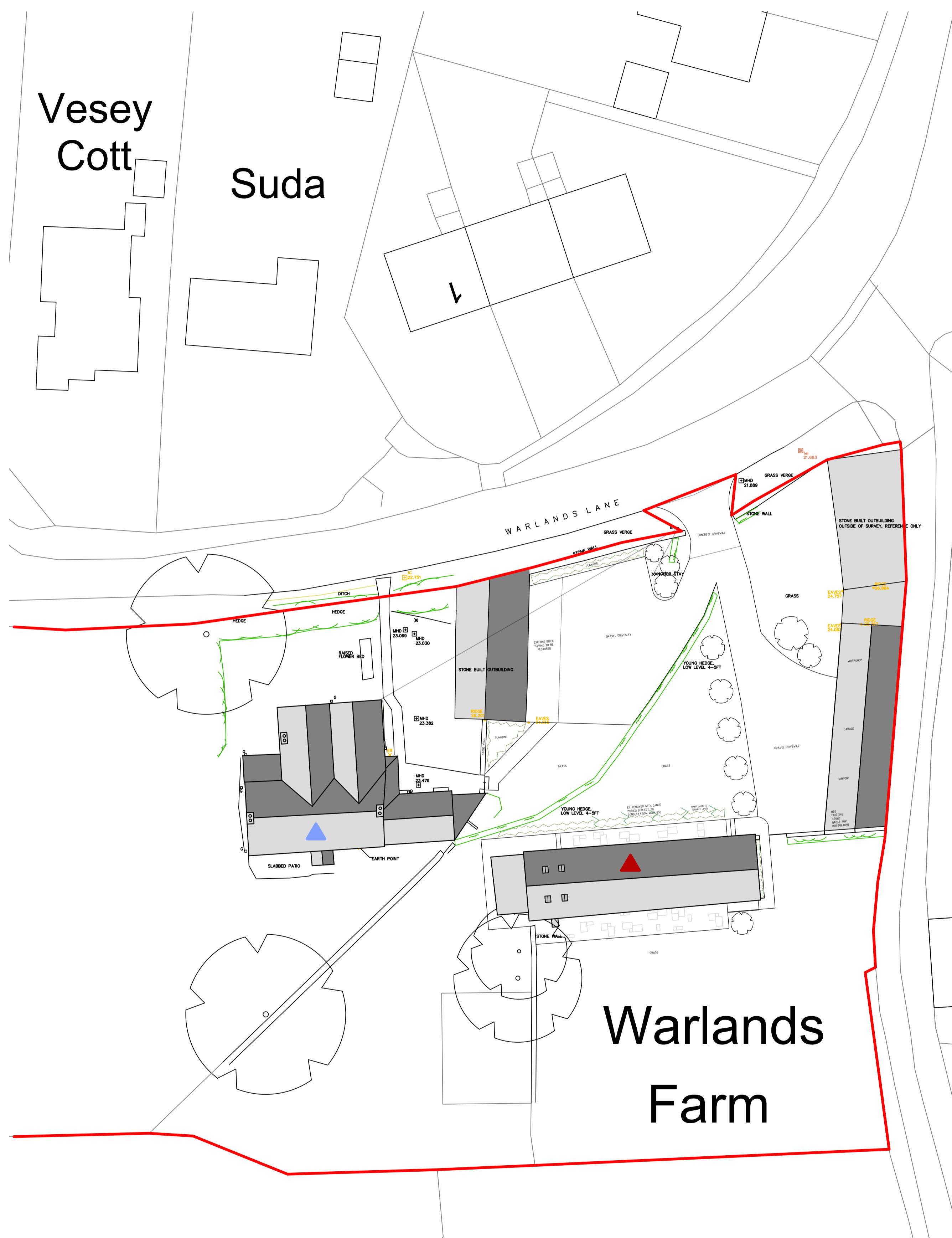
N PROPOSED BLOCK PLAN 1:500 @ A3 // 1:250 @ A1 0 5 10 15 20 25 METRES
