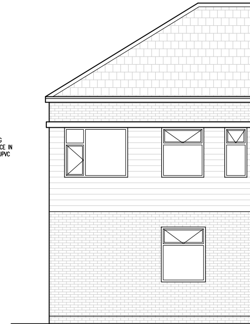
PROPOSED REAR ELEVATION 1:100 @ A3
