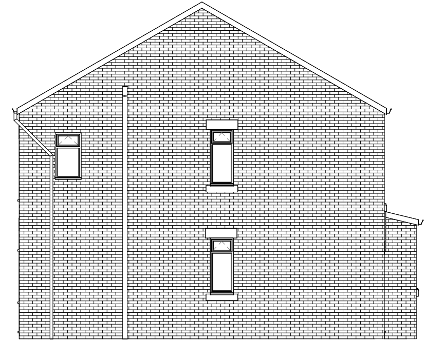
3 Gable Elevation 1 : 100
