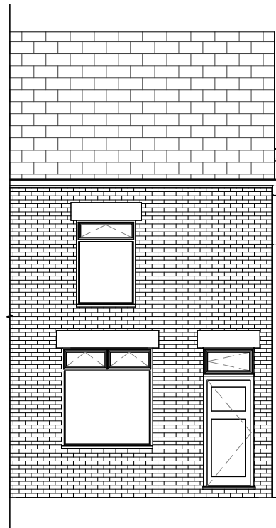
2 Front Elevation 1 : 100
