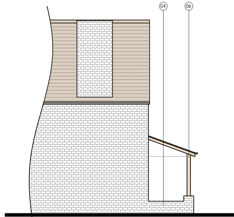
PROPOSED SIDE // WEST ELEVATION Scale - 1:100
