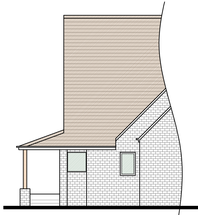
PROPOSED SIDE // EAST ELEVATION Scale - 1:100
