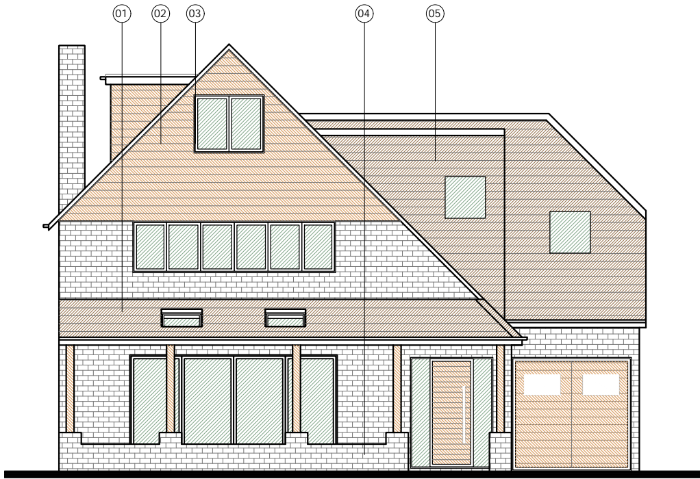
PROPOSED FRONT // SOUTH ELEVATION Scale - 1:100
