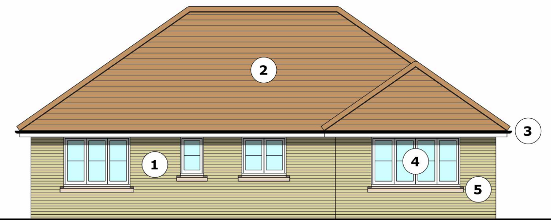
REAR ELEVATION
