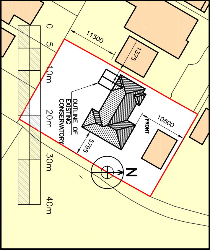
BLOCK PLAN & EXISTING ROOF PLAN
