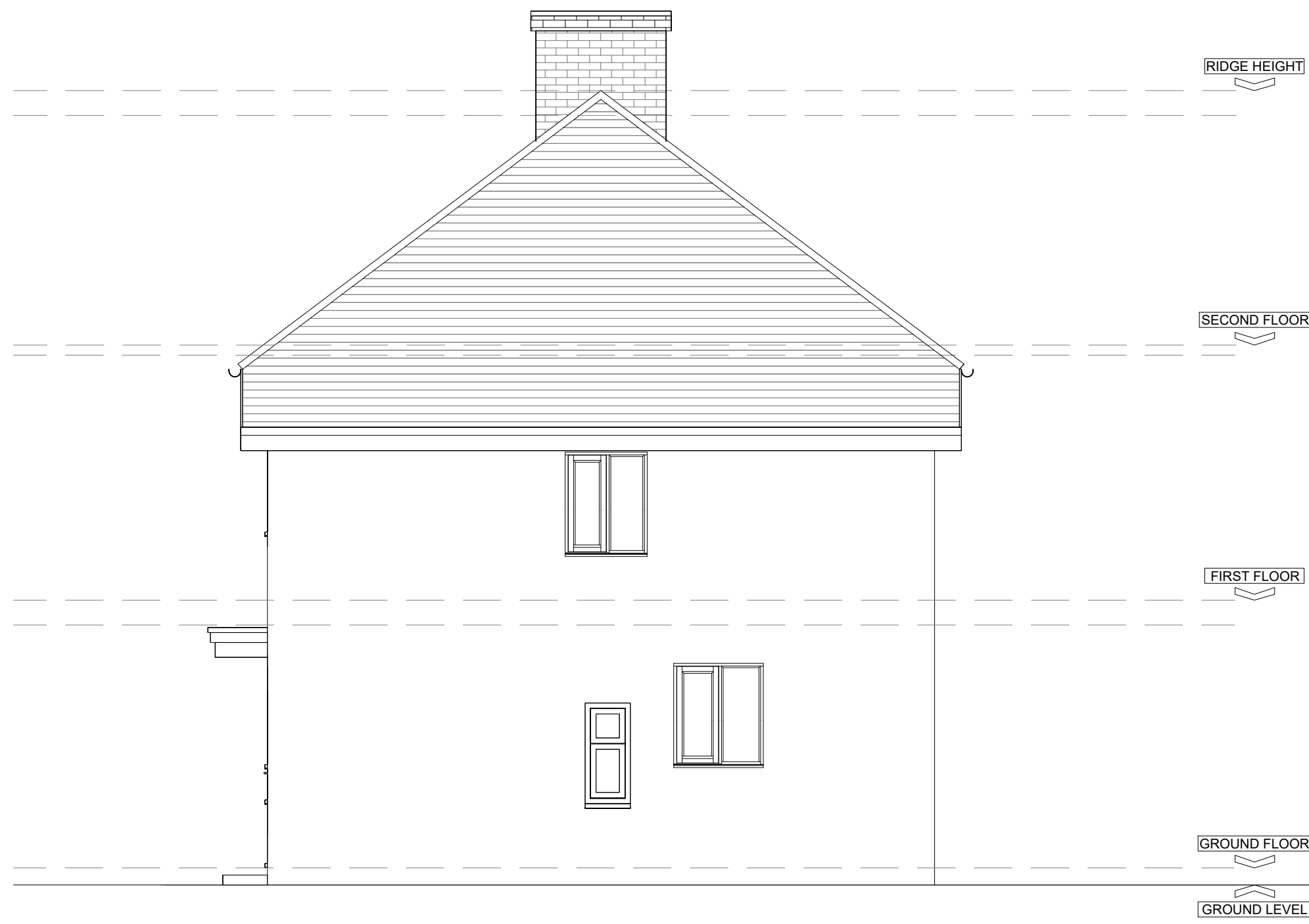
4 ELEVATION - SIDE EXISTING 1:50 @ A1
