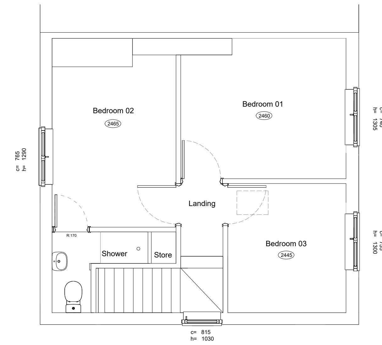
2 FIRST FLOOR EXISTING 1:50 @ A1 FF Existing Area = 32 sqm
