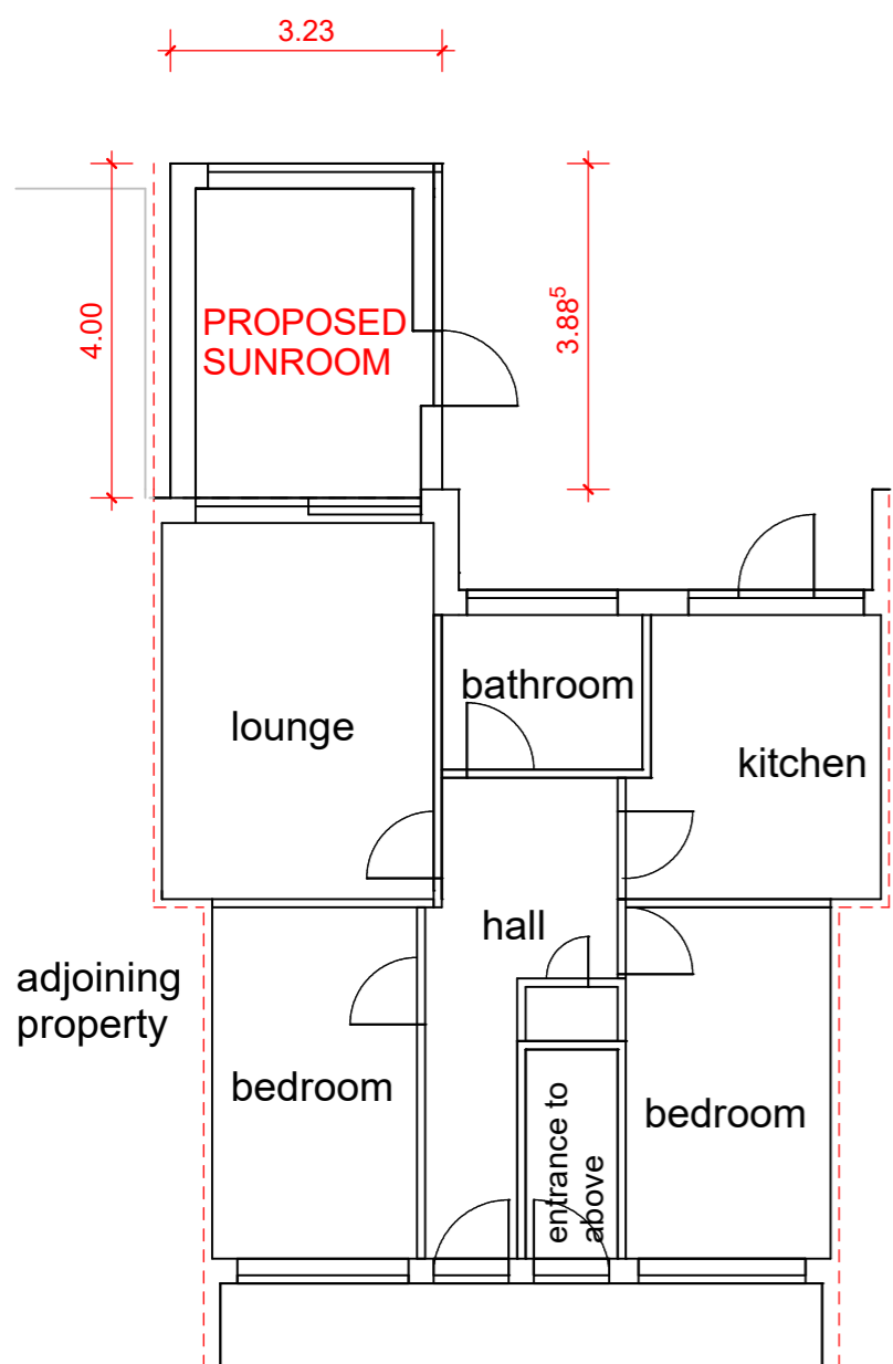
FLOOR LAYOUT
