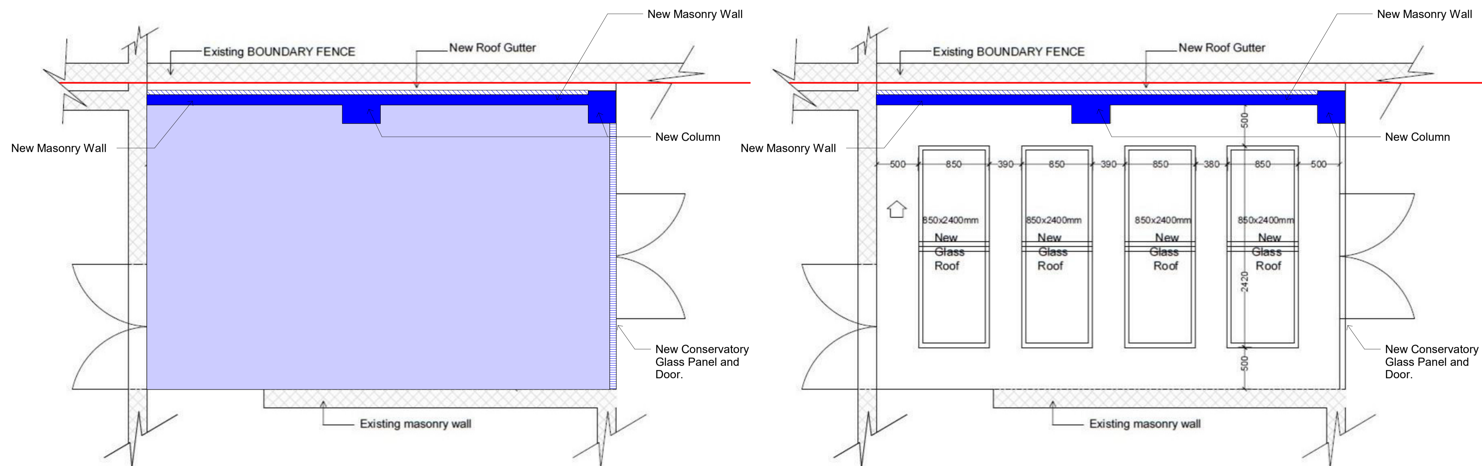
GLASS ROOF DETAIL NTS
