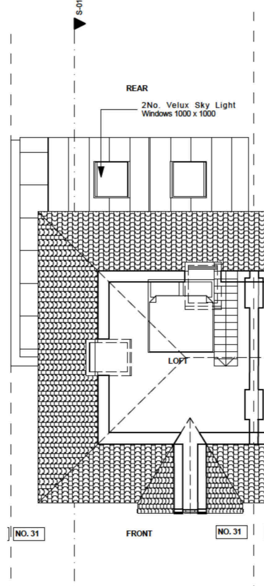
3 - Loft Floor Plan 1:100
