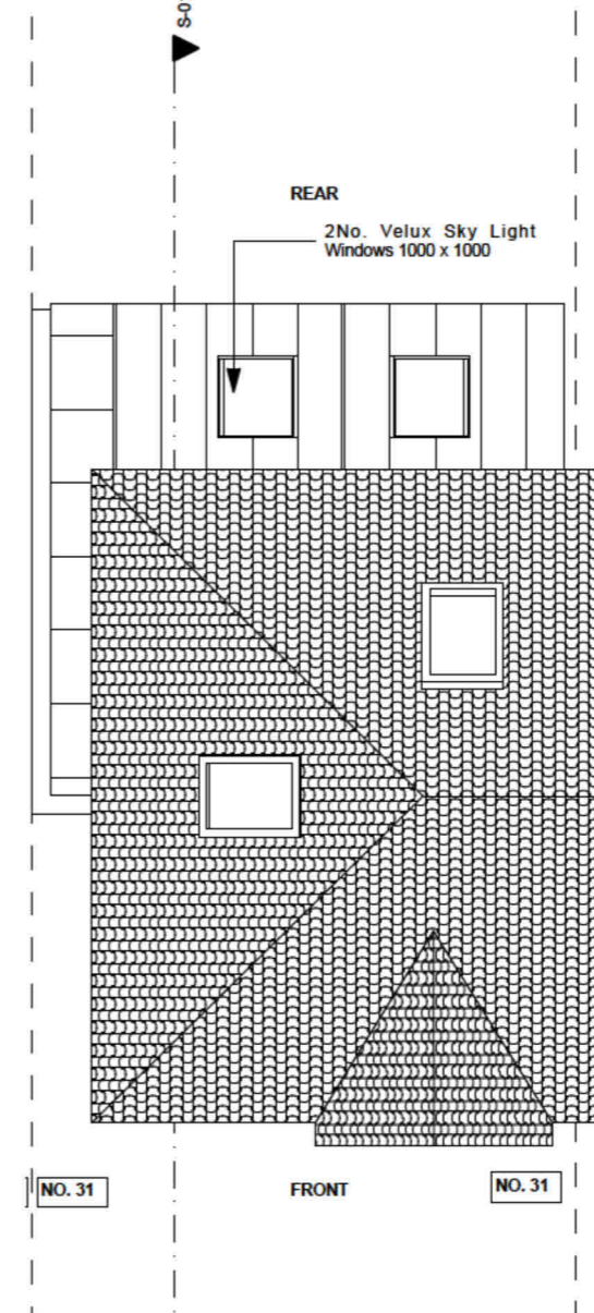
4 - Roof Floor Plan 1:100
