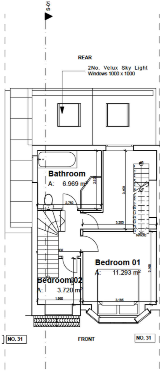
2 - First Floor Plan 1:100
