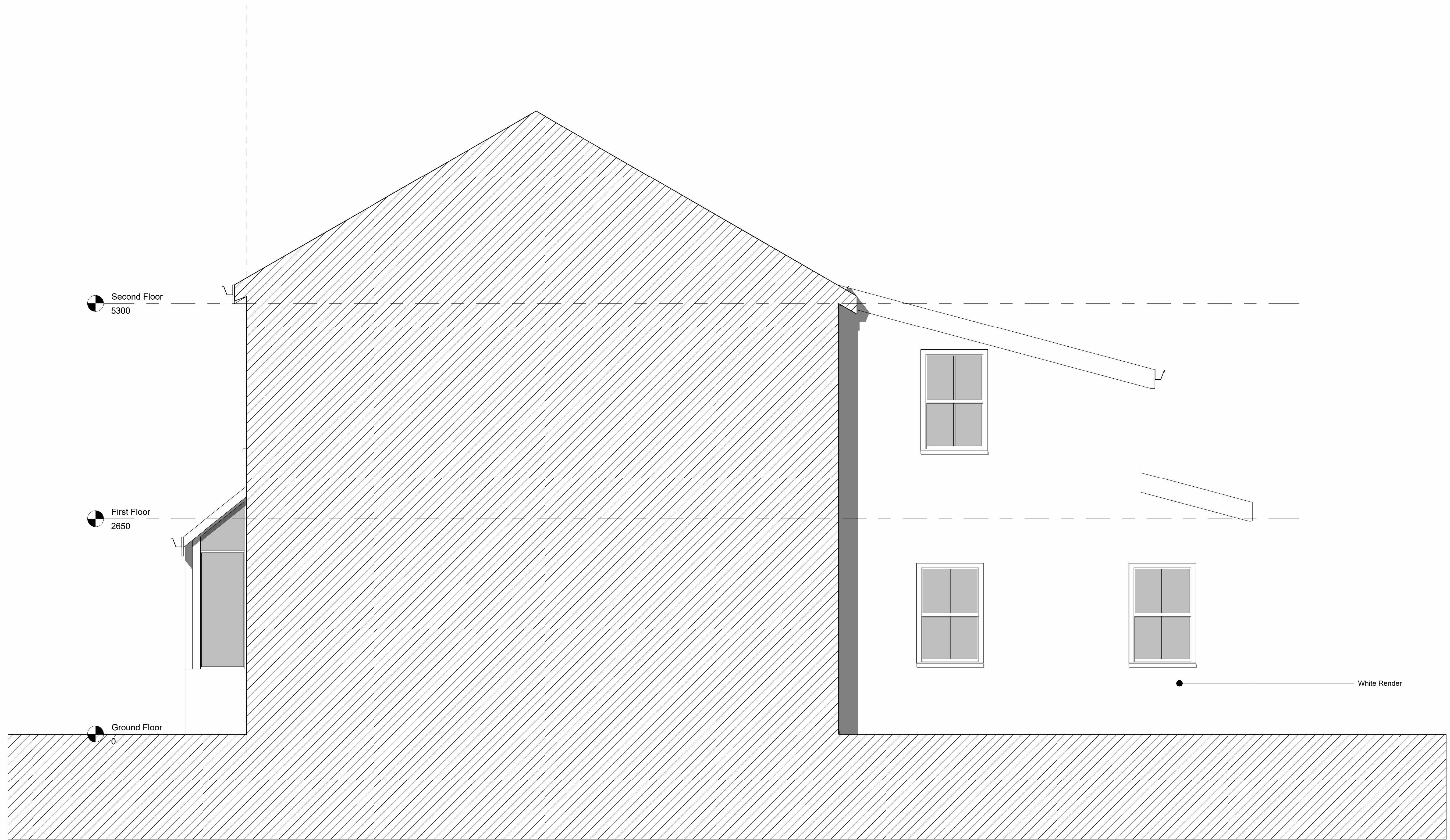
1 Existing Side Elevation 1 : 25
