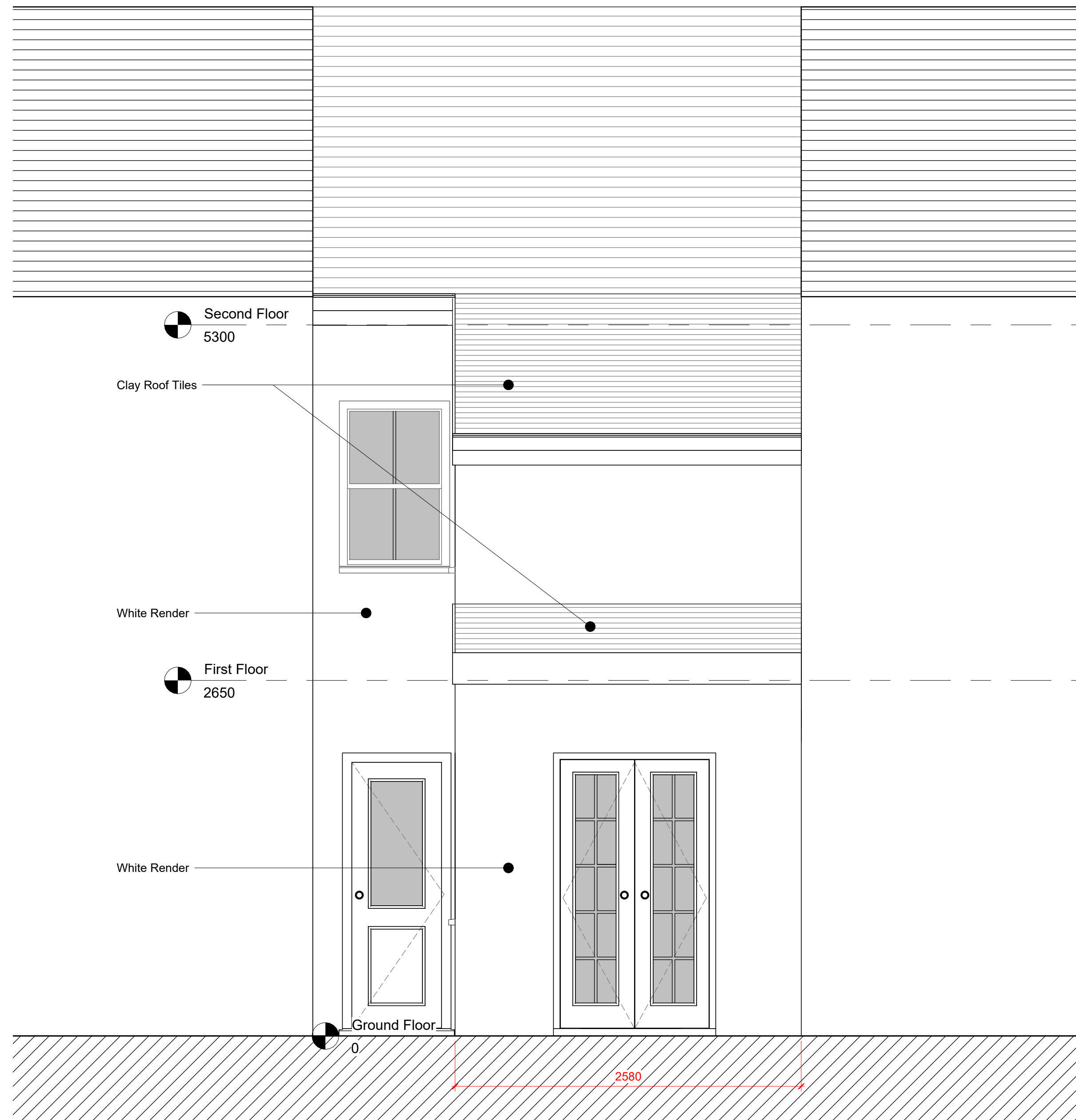
Existing Rear Elevation 1 : 25
