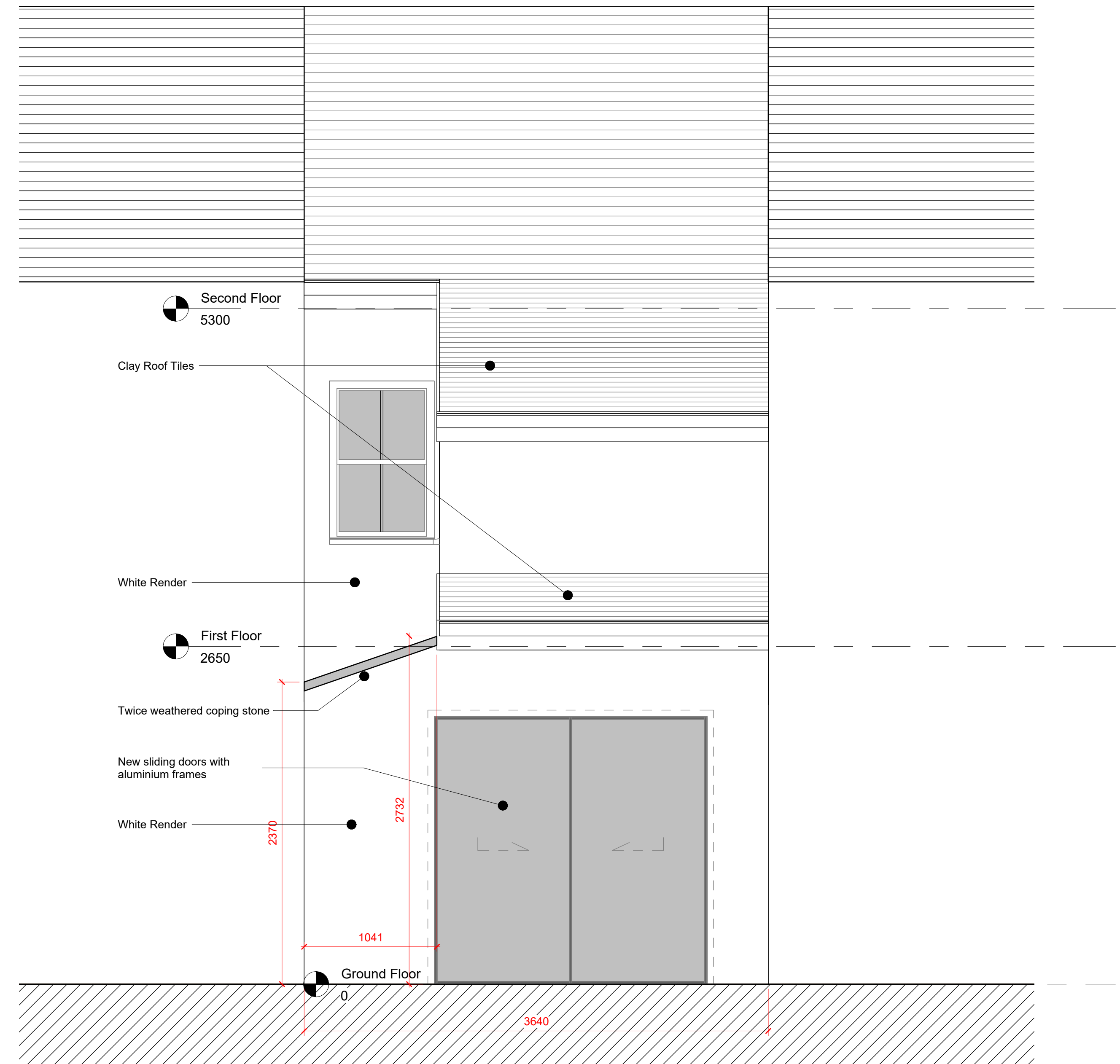
Proposed Rear Elevation 1 : 25
