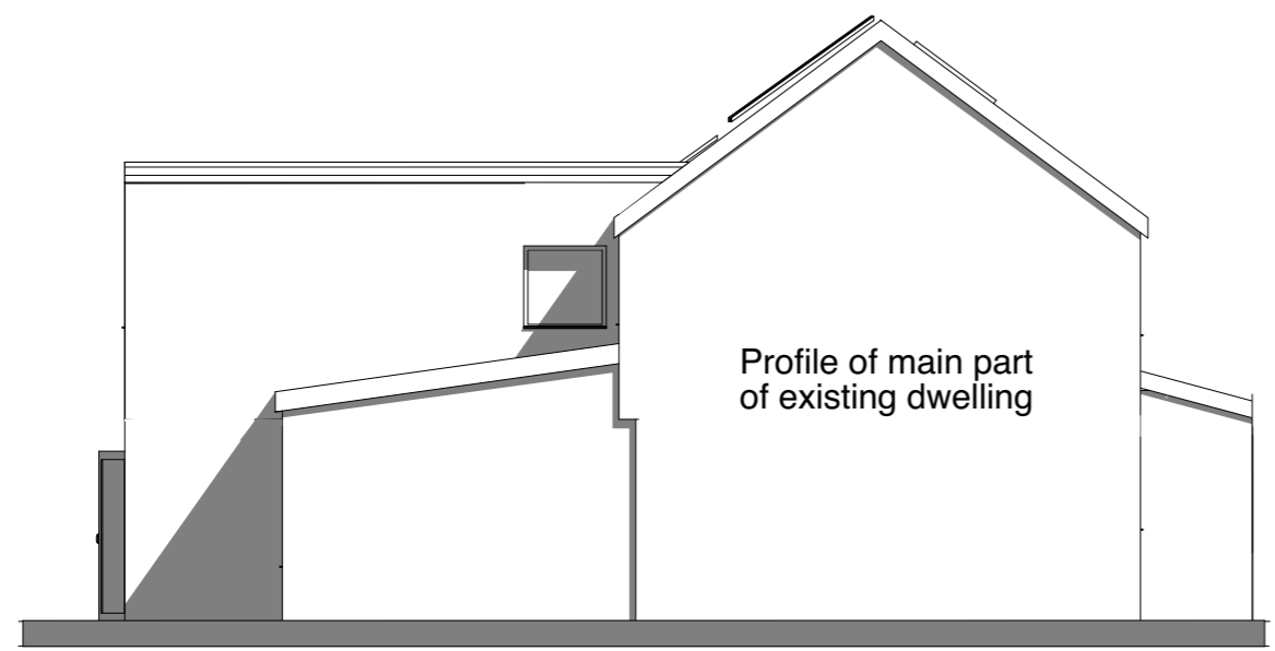
East Elevation 1:100
