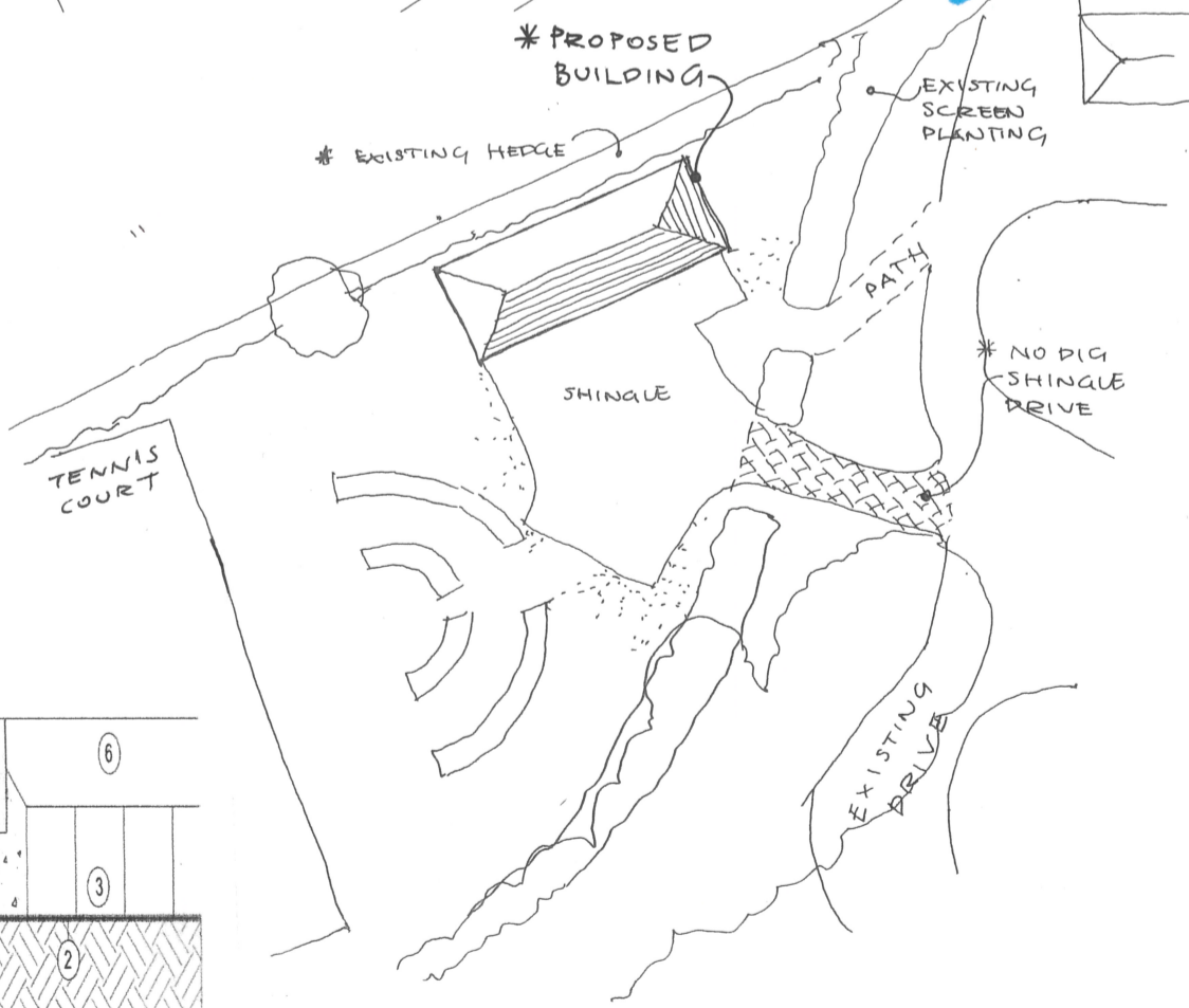
'No Dig' Construction / Ground Protection Detail
