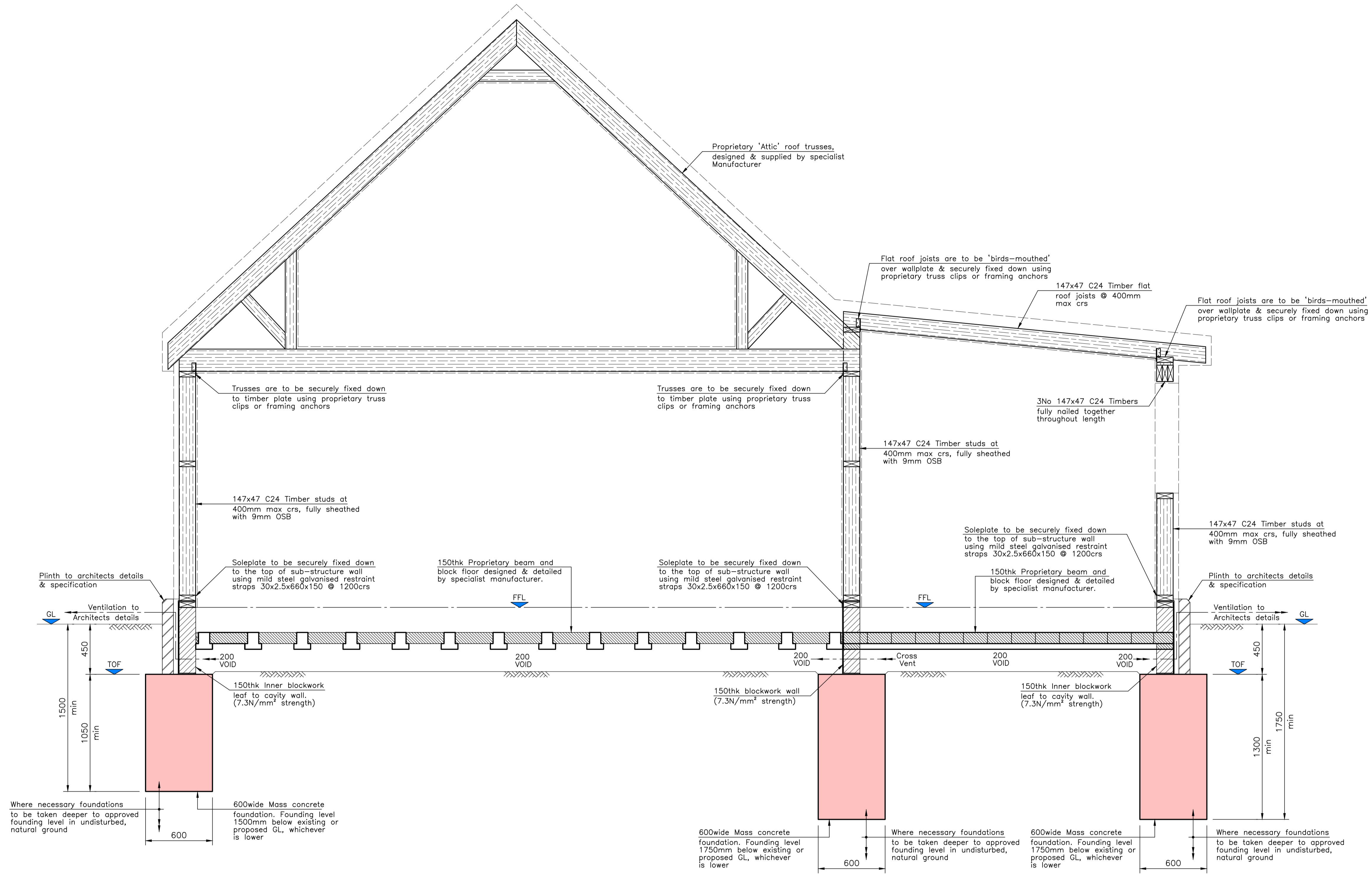
SECTION X-X
