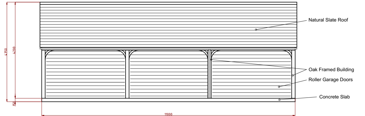
PROPOSED SOUTH WEST FACING ELEVATION
