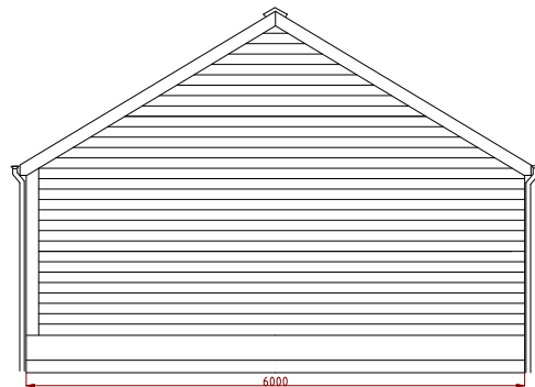
PROPOSED SOUTH EAST FACING ELEVATION
