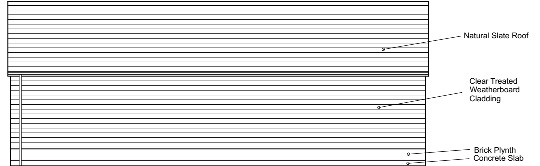
PROPOSED NORTH EAST FACING ELEVATION
