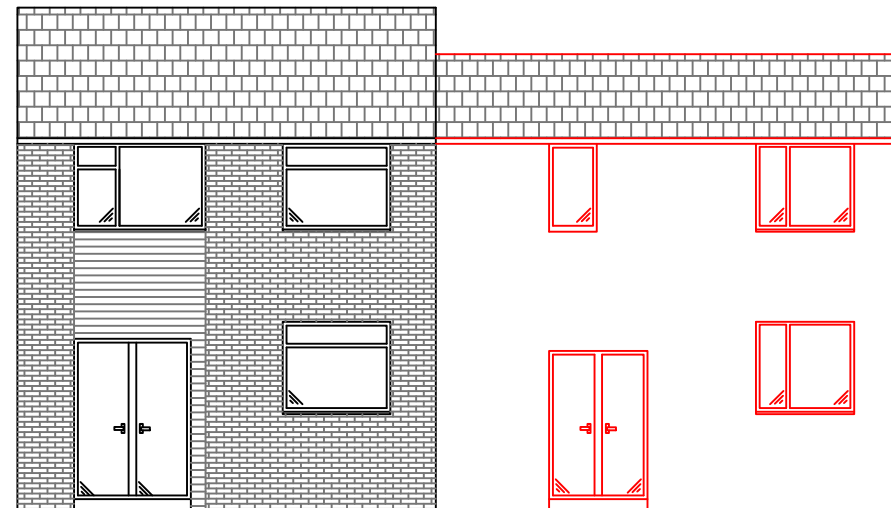
PROPOSED NEW DWELLING REAR ELEVATION
