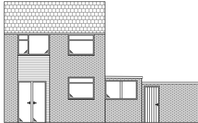
EXISTING 1 PARKHILL REAR ELEVATION
