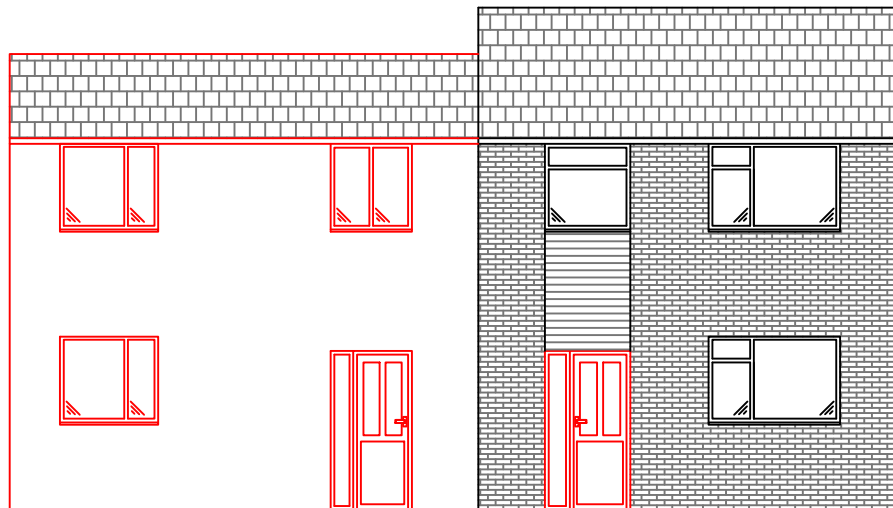
PROPOSED NEW DWELLING FRONT ELEVATION
