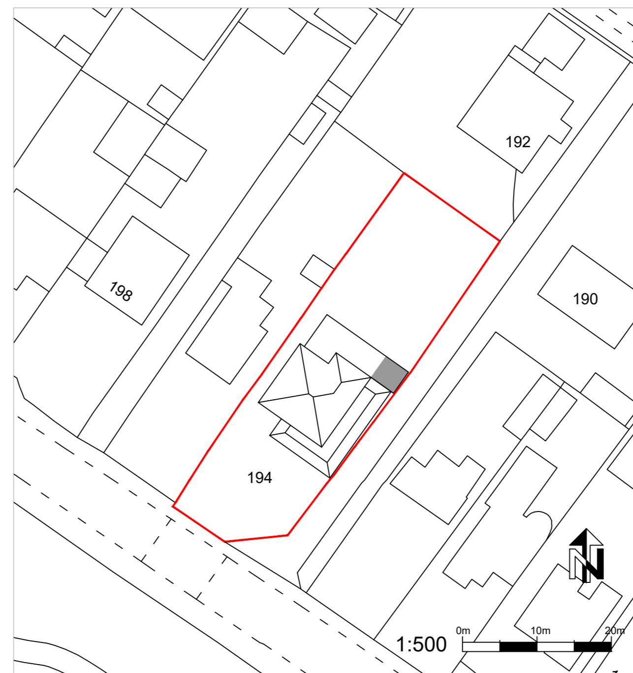
Block Plan 1:500
