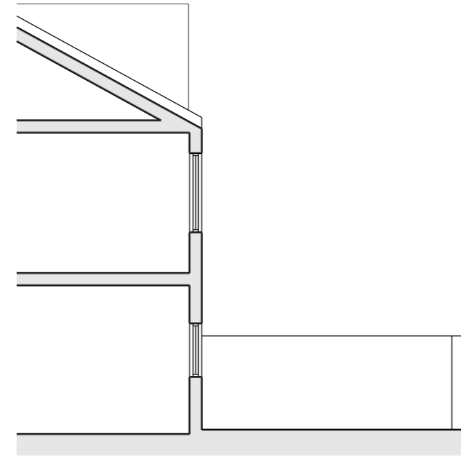
Existing Section AA @ 1:100
