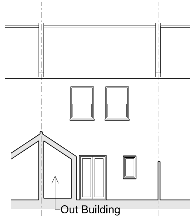
Existing Section BB @ 1:100
