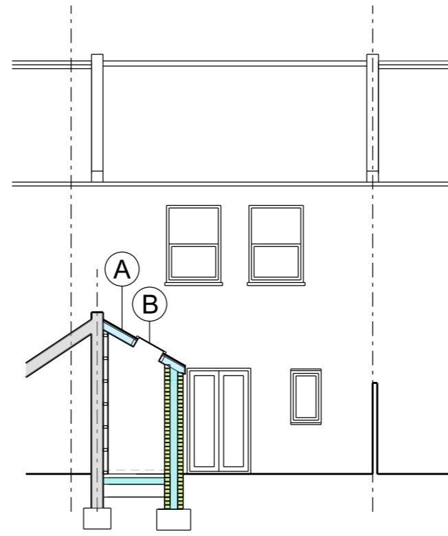
Proposed Section BB @ 1:100
