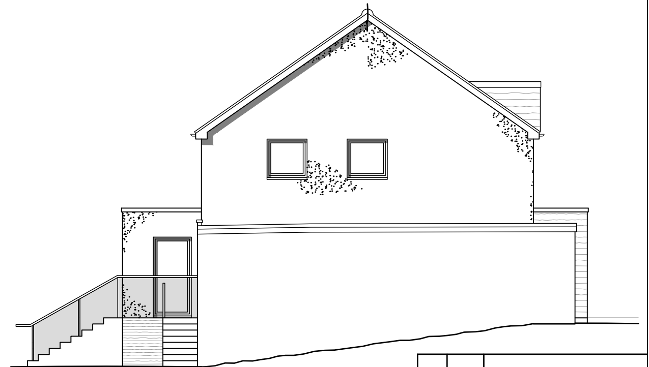
West Elevation
