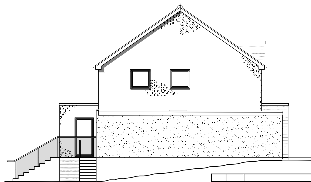
West Elevation
