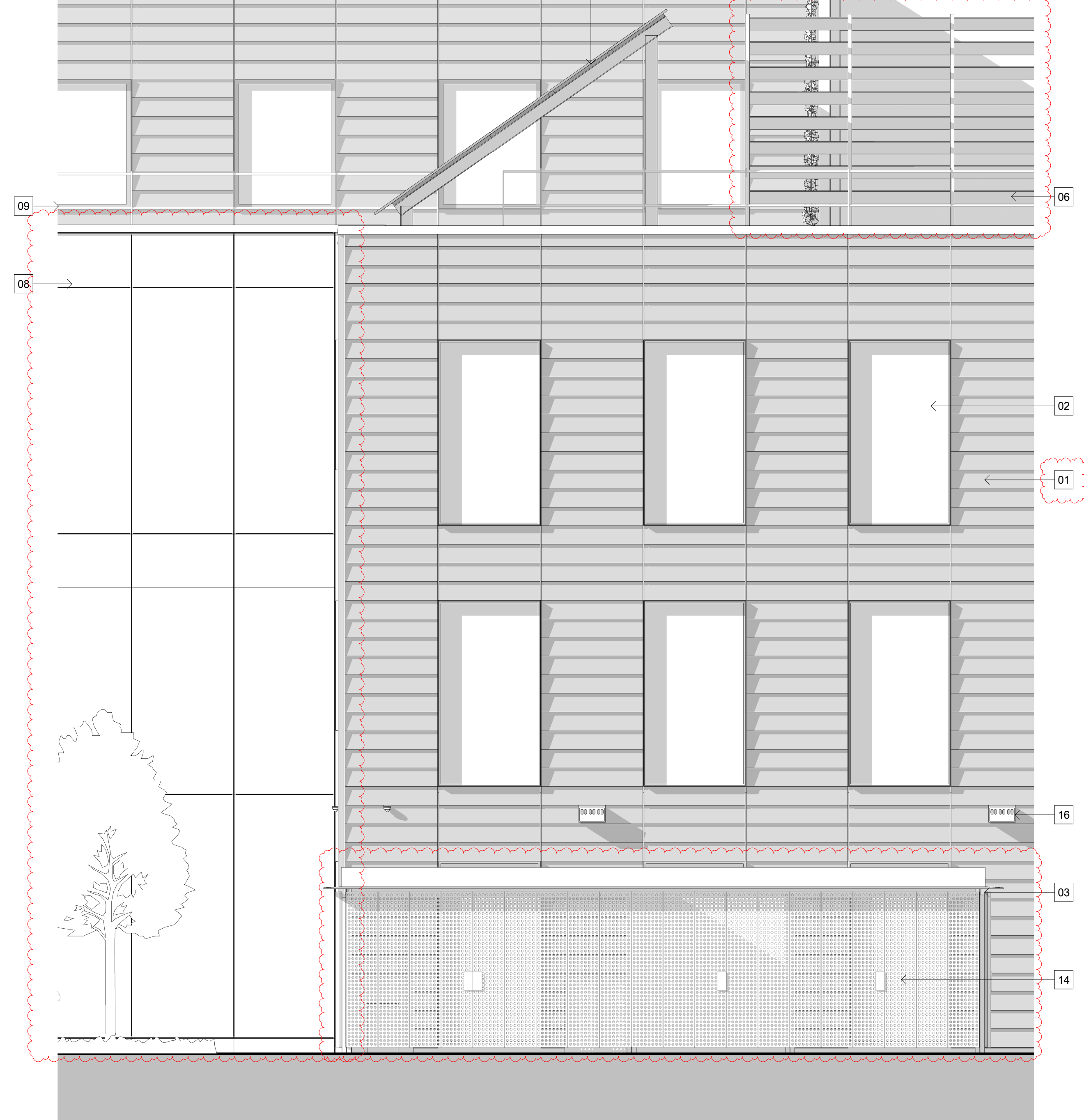
2 South East Facade Elevation 1 : 50
