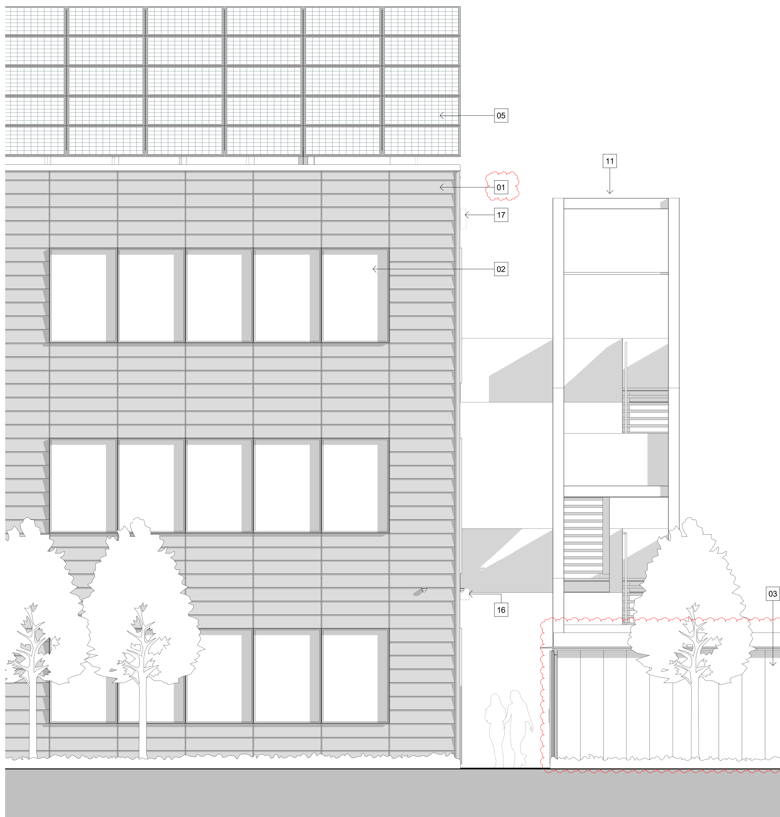
1 South West Facade Elevation 1 : 50
