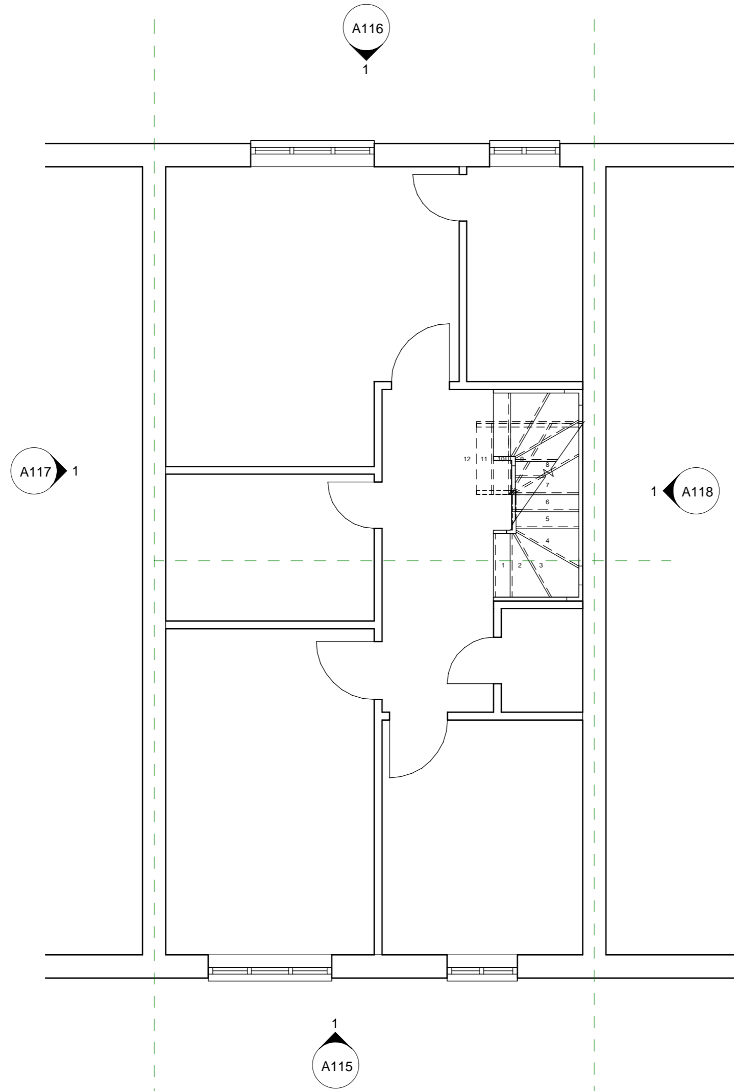
1 Proposed Level 1 - First Floor 1 : 50
