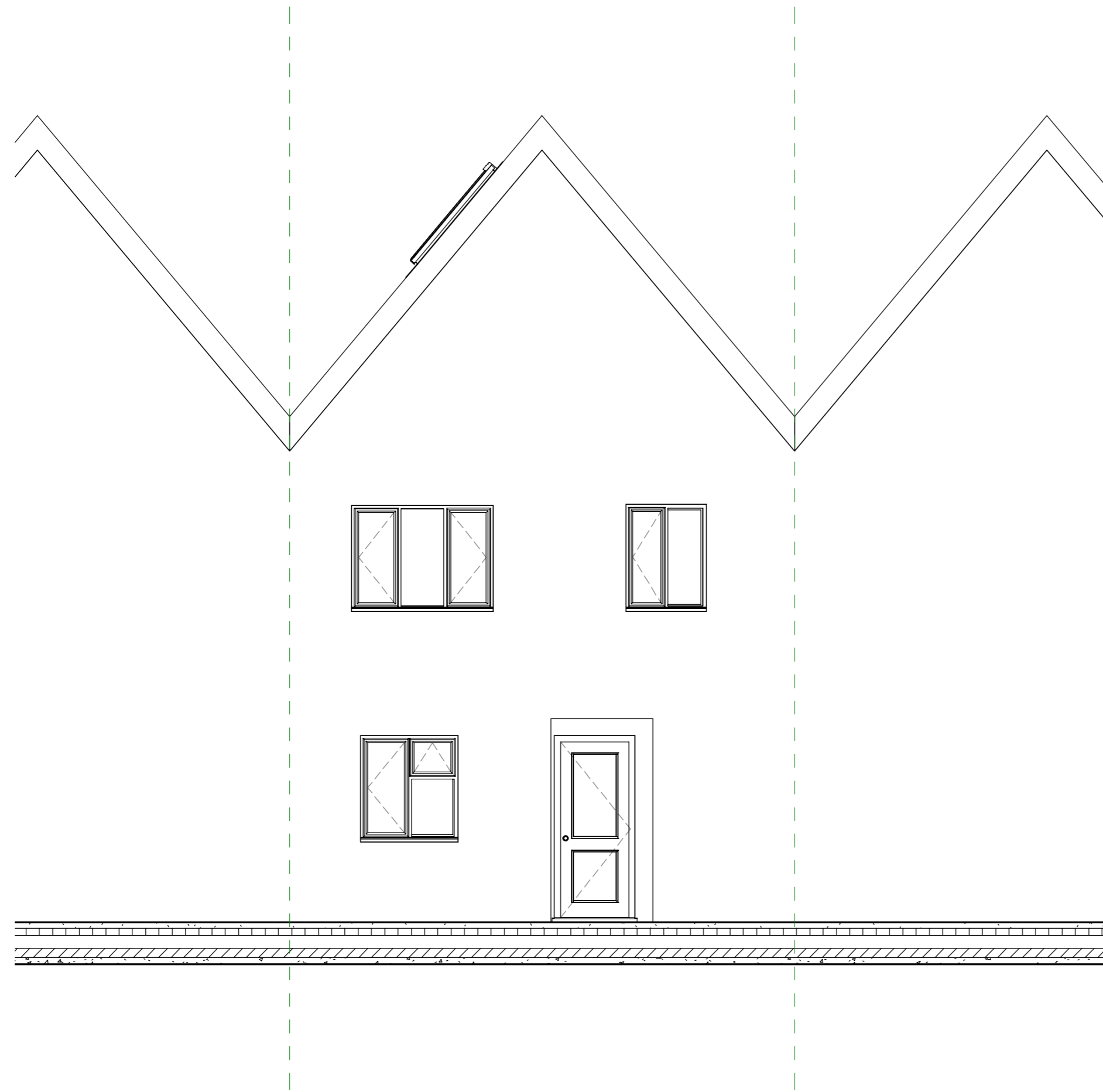
1 Proposed Front Elevation 1 : 50
