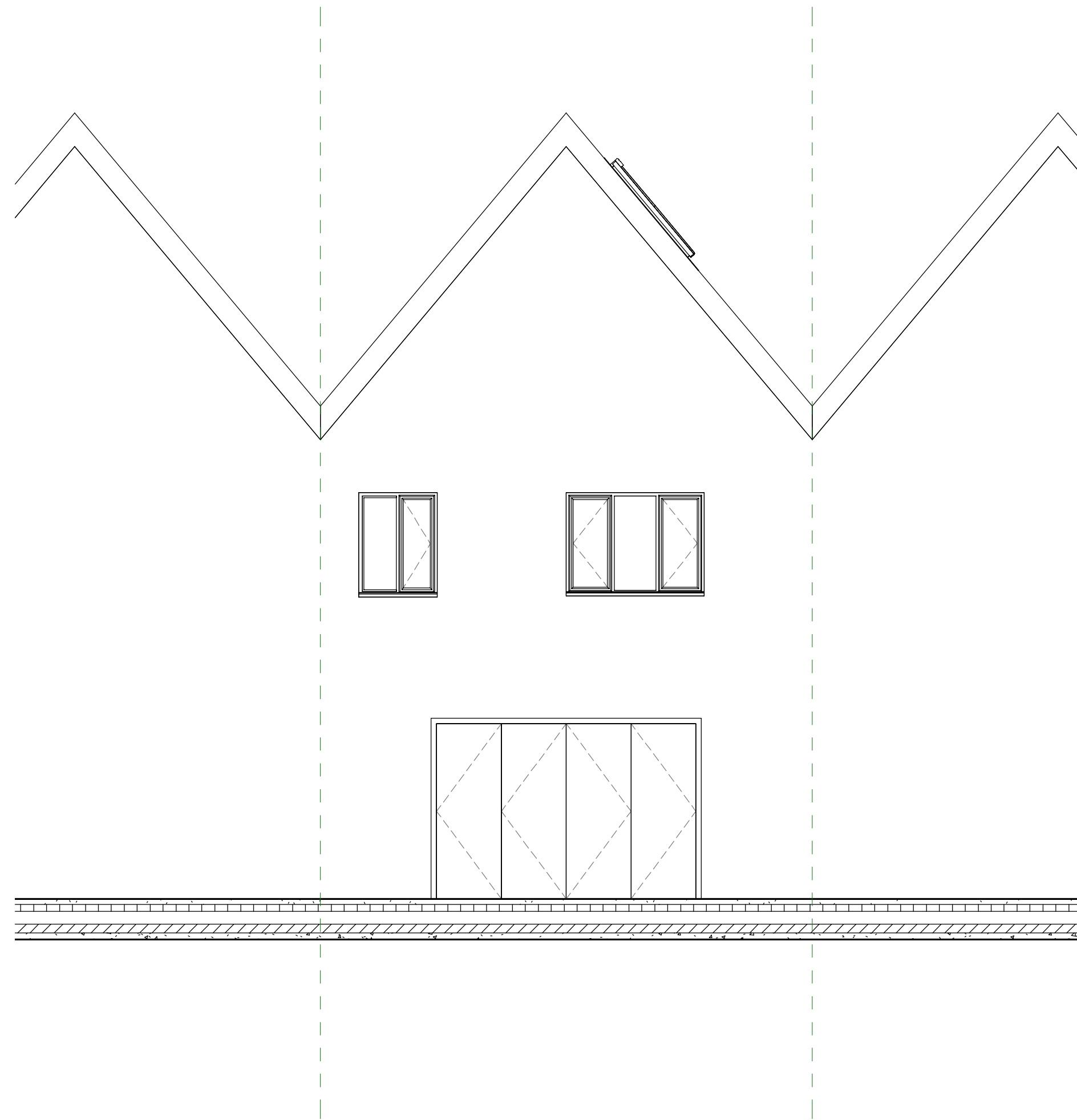
1 Proposed Rear Elevaton 1 : 50
