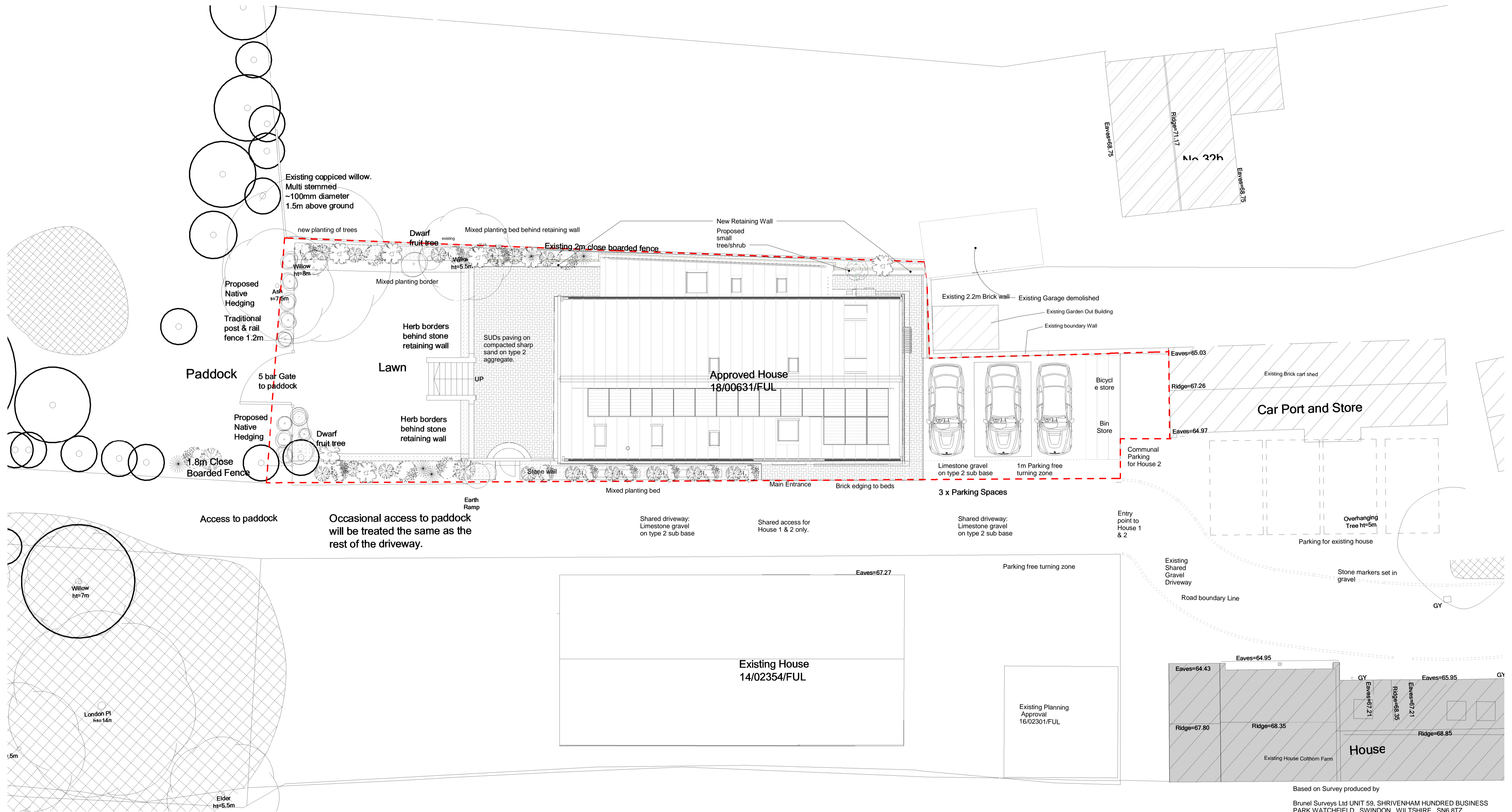
1 Landscape Plan 1:100
