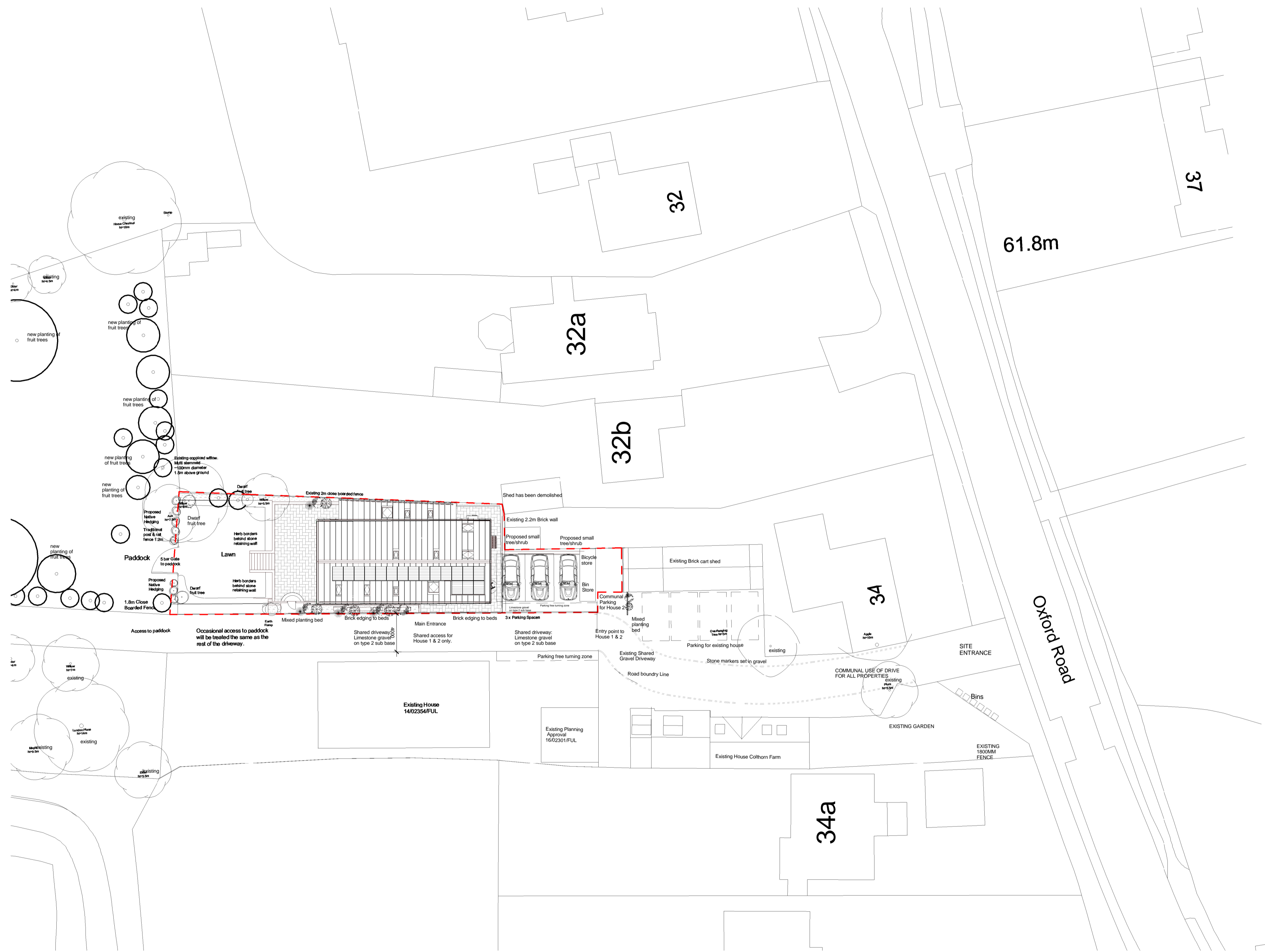
1 Block Plan 1:250 0m 5m 10m 15m 20m 25m VISUAL SCALE 1:250
