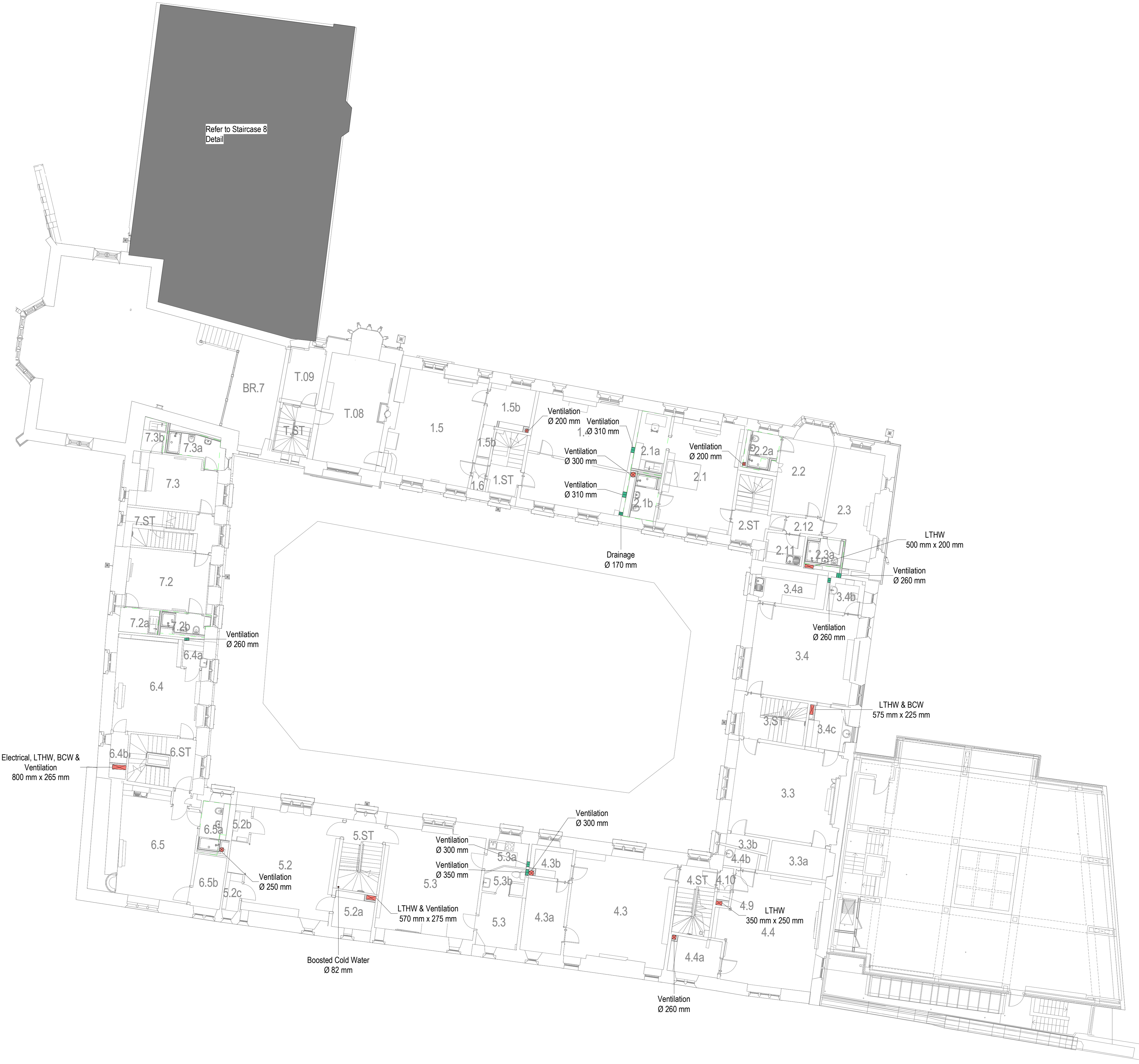
1 500 - Builders Work in Connection - Level 01 (Old Quad) 1 : 100
