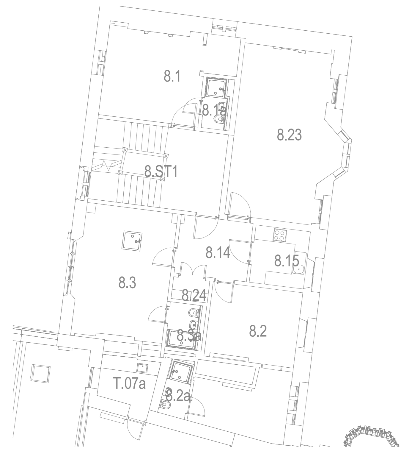
2 500 - Builders Work in Connection - Level 01 (Staircase 8) 1 : 100
