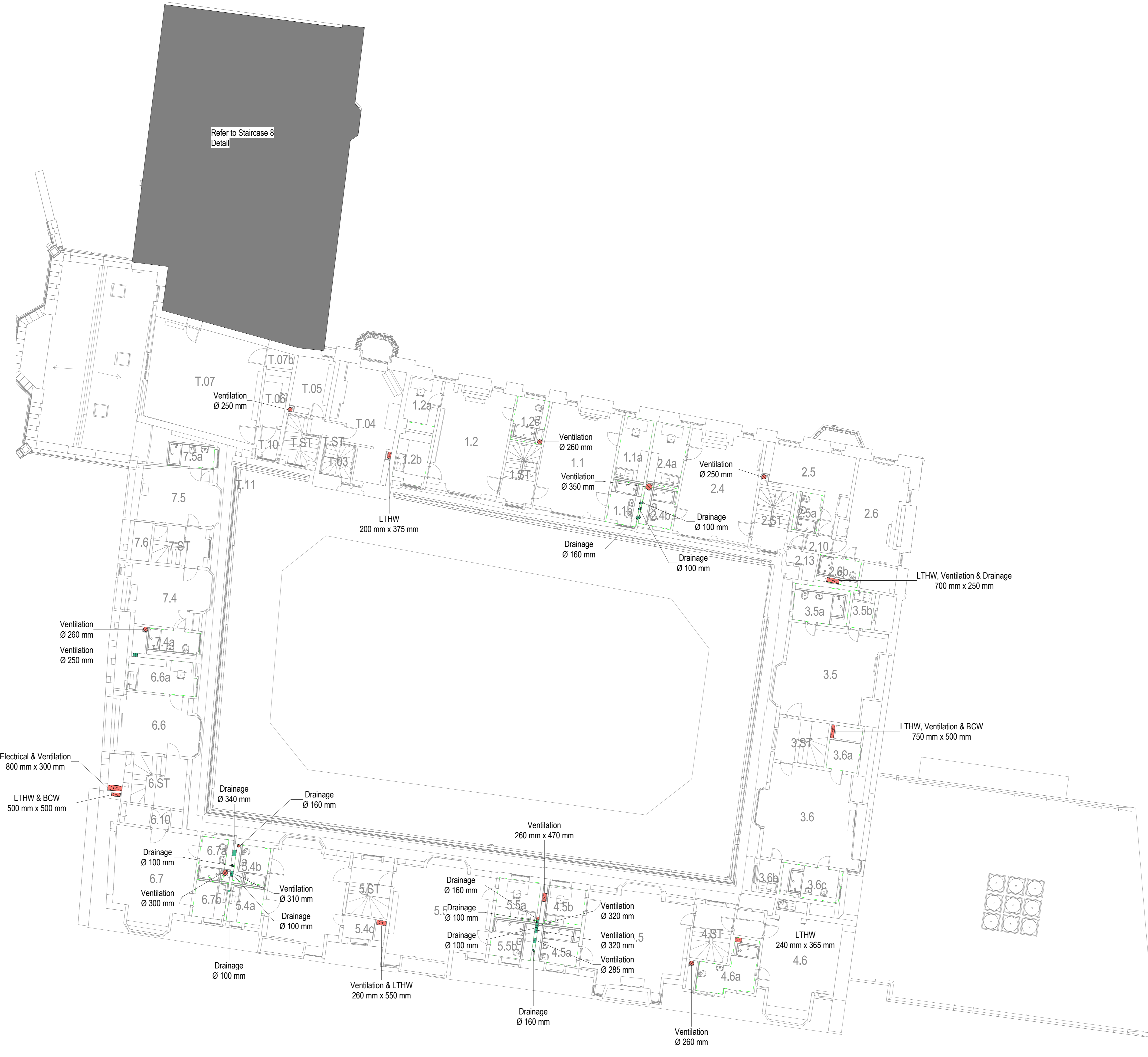
1 500 - Builders Work in Connection - Level 02 (Old Quad) 1 : 100
