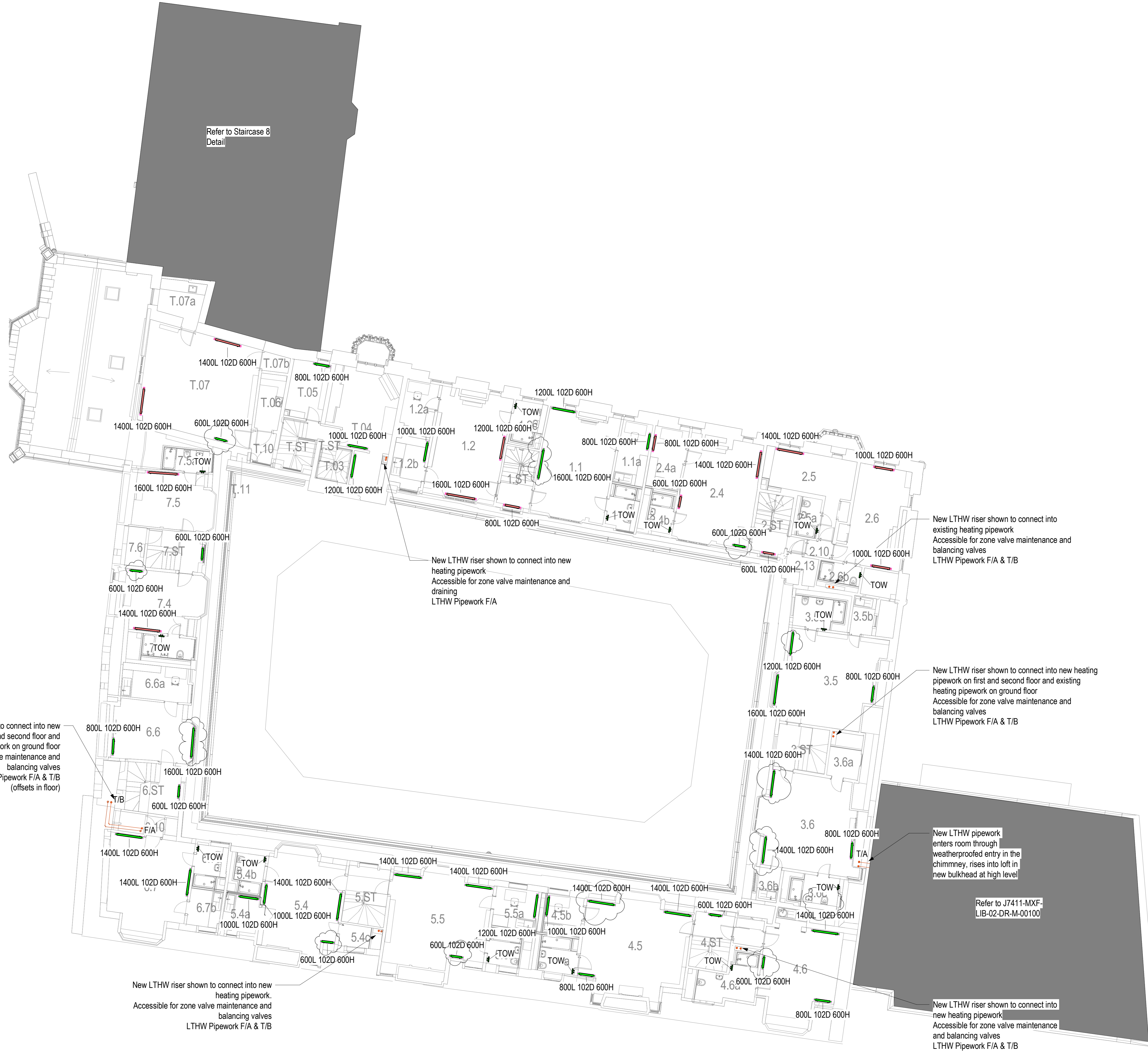
1 500 - Heating (Detail) - Level 02 - Old Quad 1 : 100
