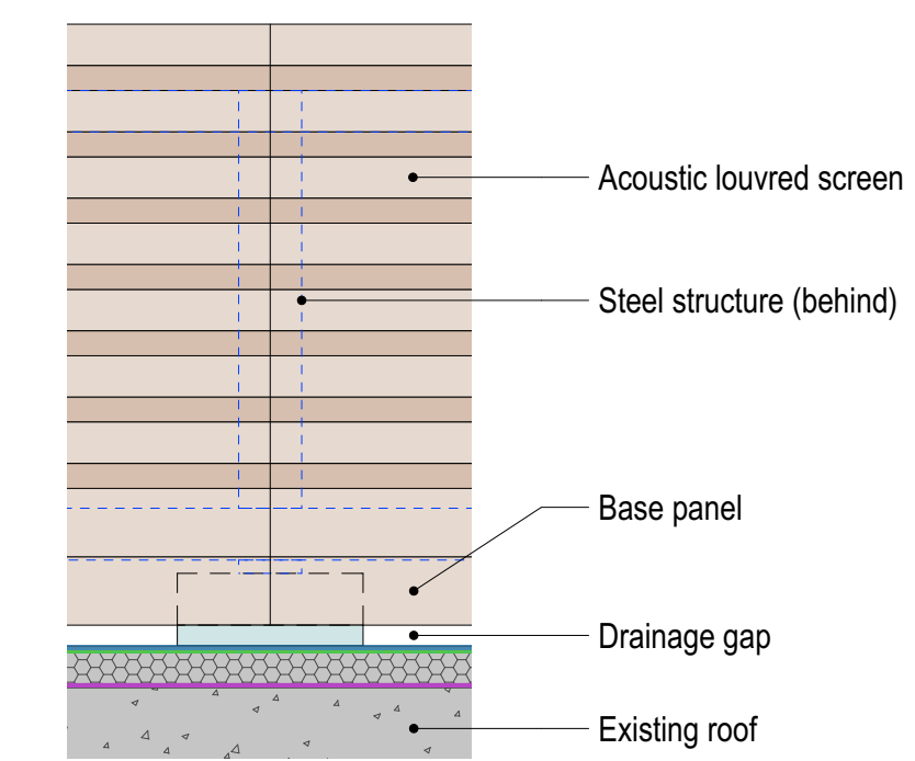
McGowin Library ASHP Enclosure D04 - Typical Detailed Elevation 1:20 @ A1
