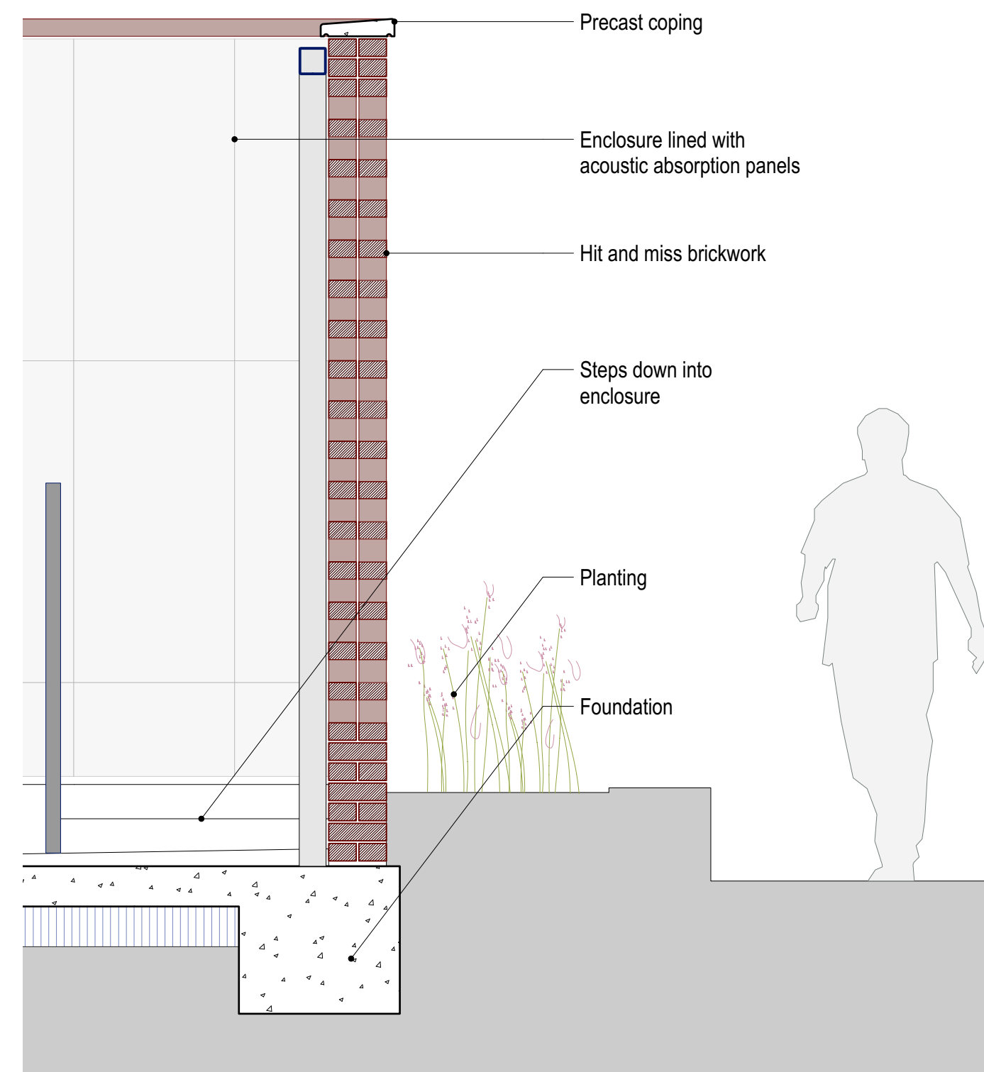
North Quad ASHP Enclosure D01 - West Elevation Section 1:20 @ A1
