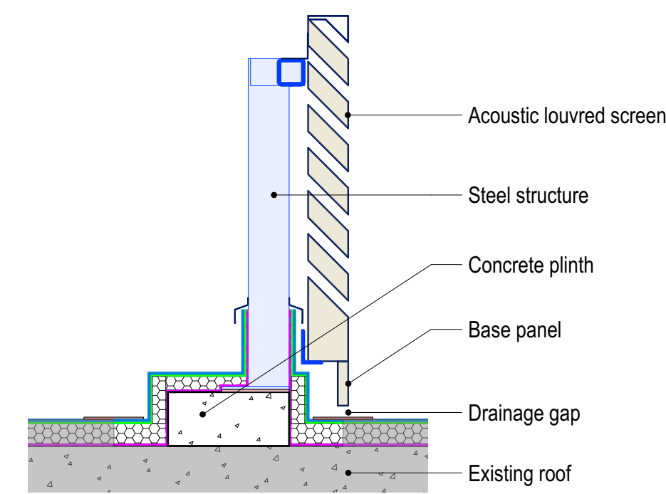
McGowin Library ASHP Enclosure D03 - Typical Section 1:20 @ A1
