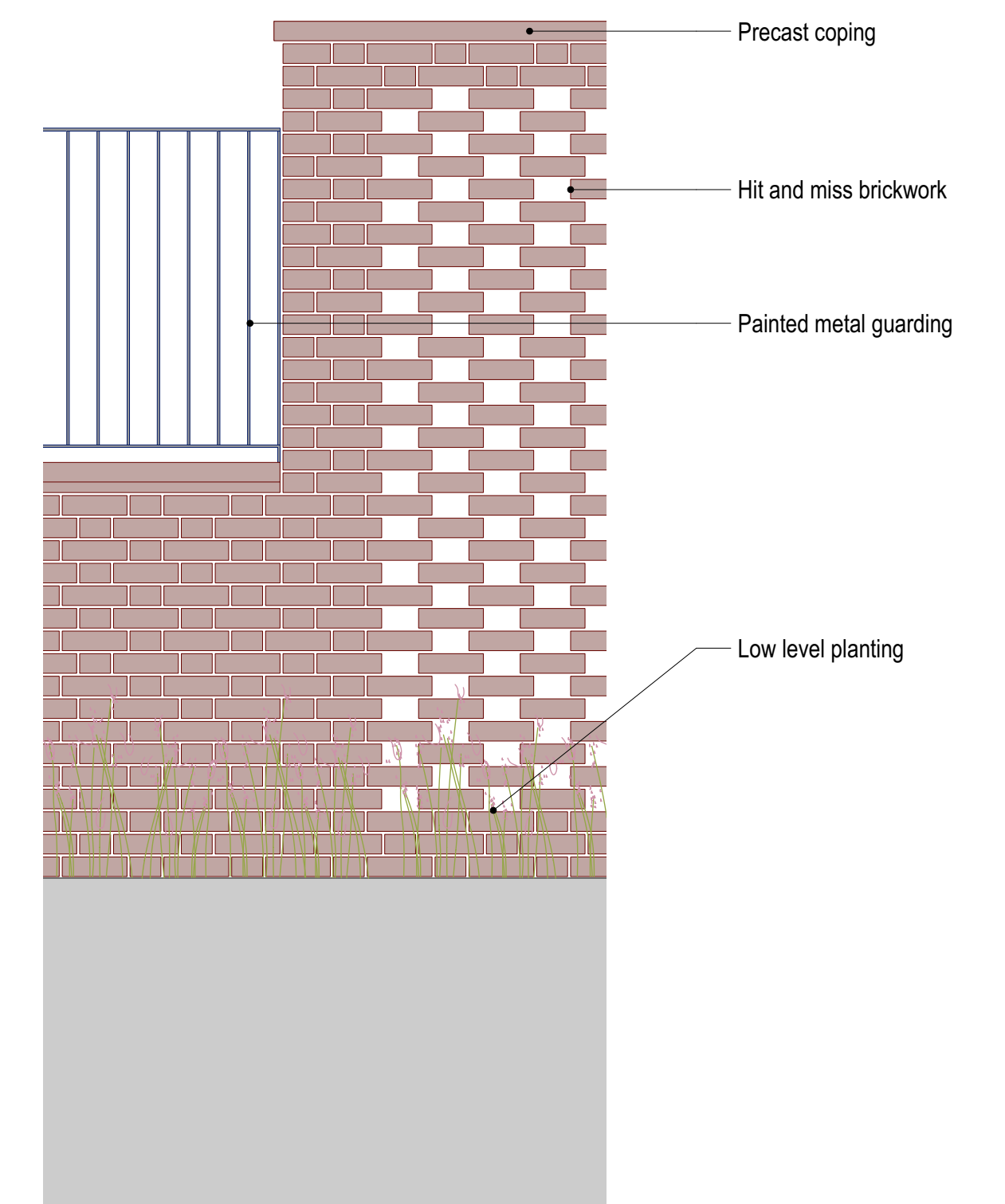
North Quad ASHP Enclosure D02 - West Elevation Detail 1:20 @ A1
