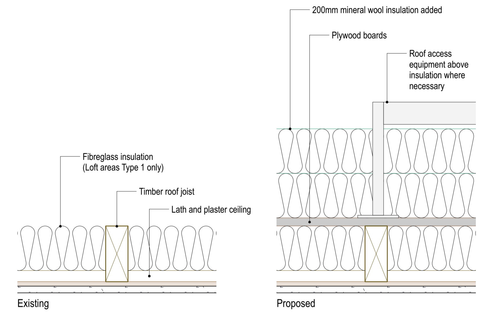
Detail 01 Existing and proposed loft insulation 1:5@A1
