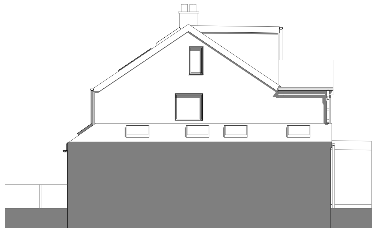
Side (South)
