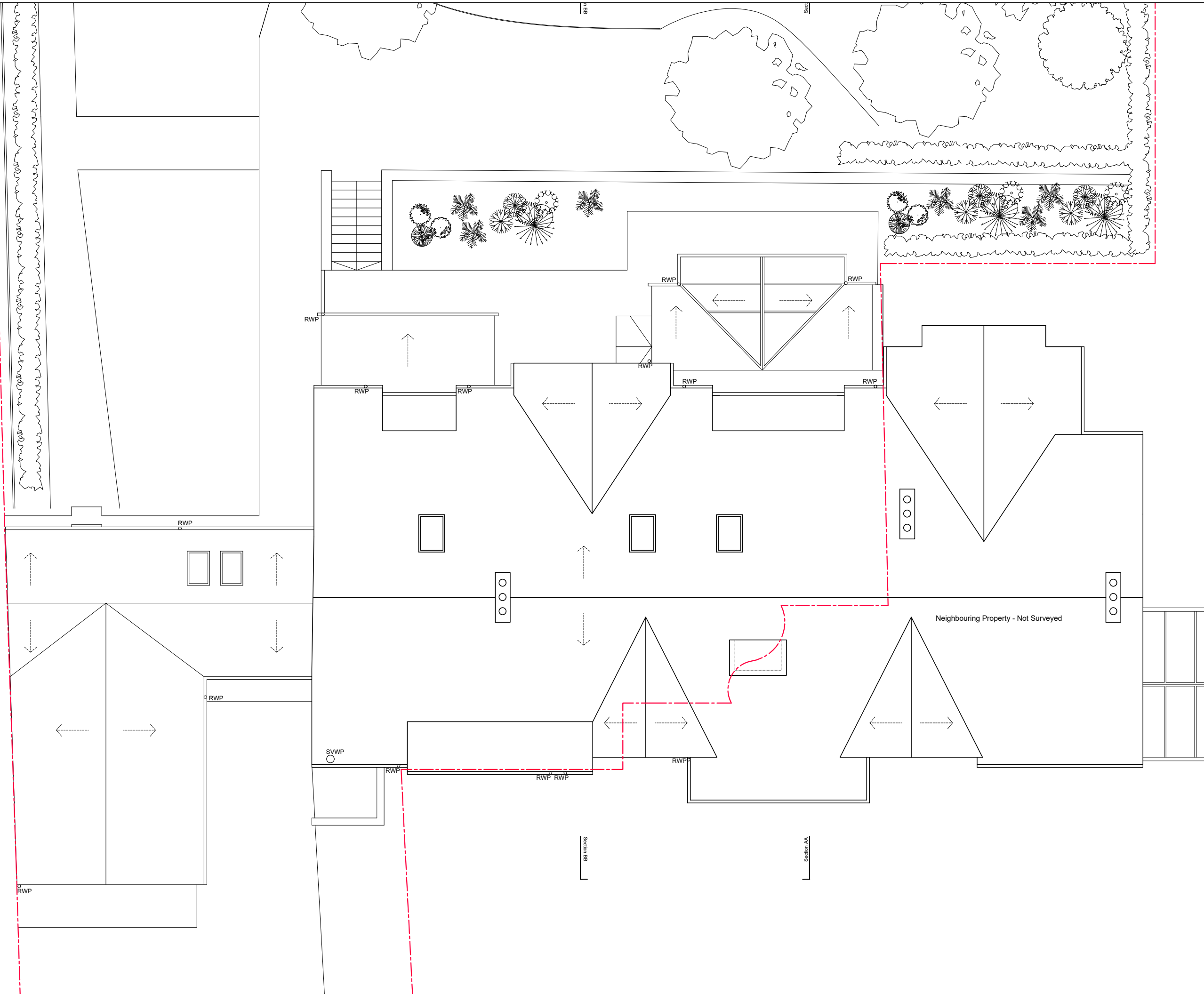
Roof Plan as Existing @ 1:100
