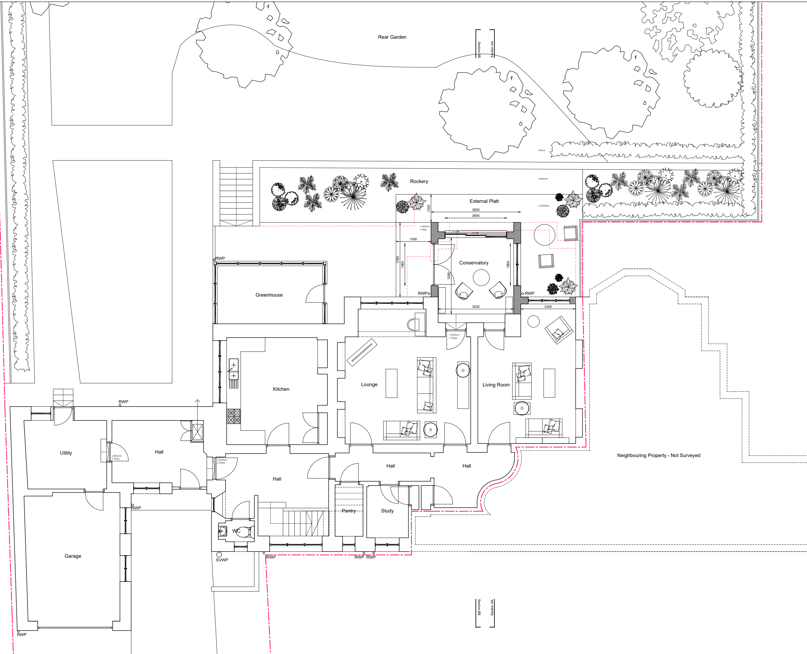
Ground Floor Plan as Proposed @ 1:100
