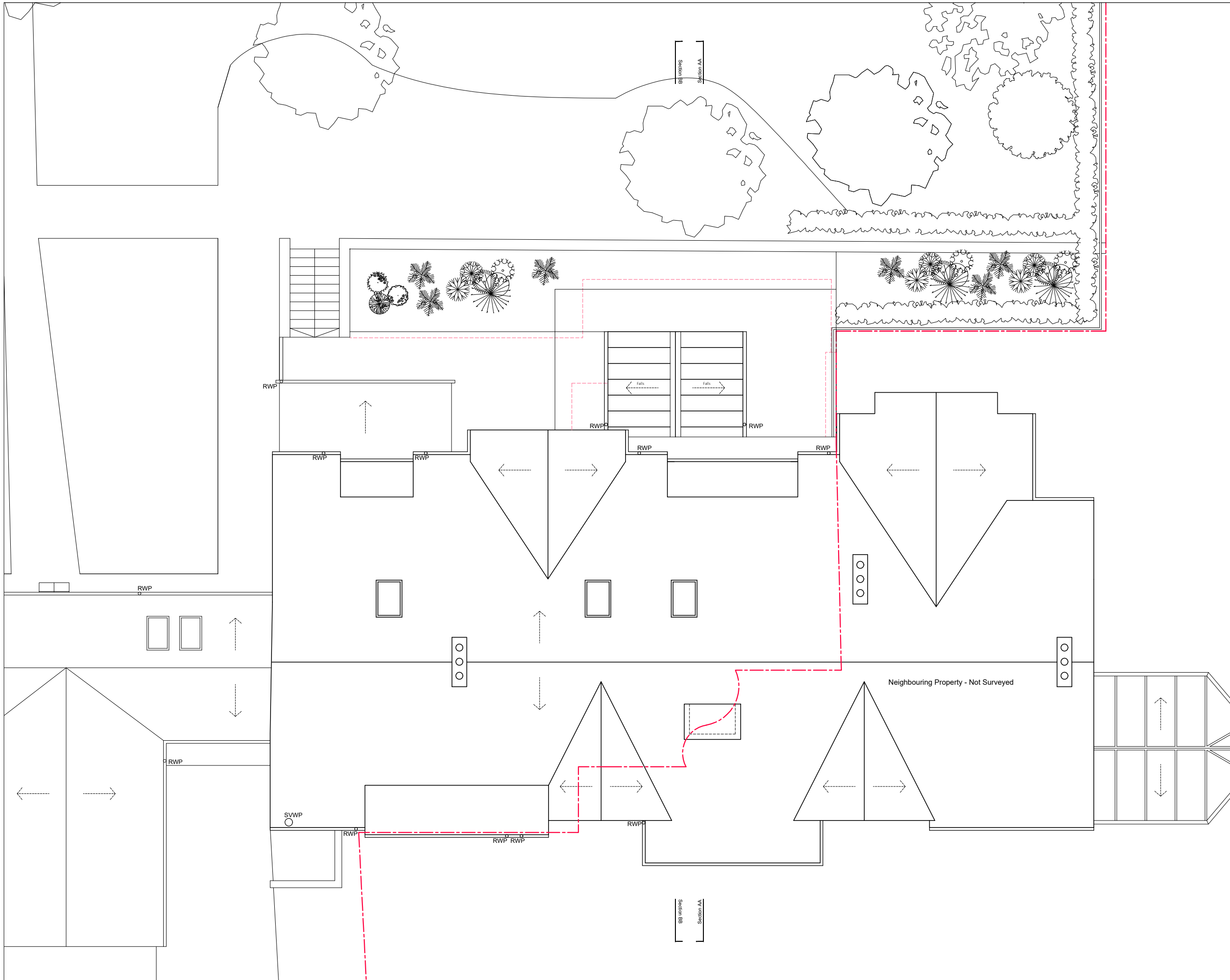
Roof Plan as Proposed @ 1:100
