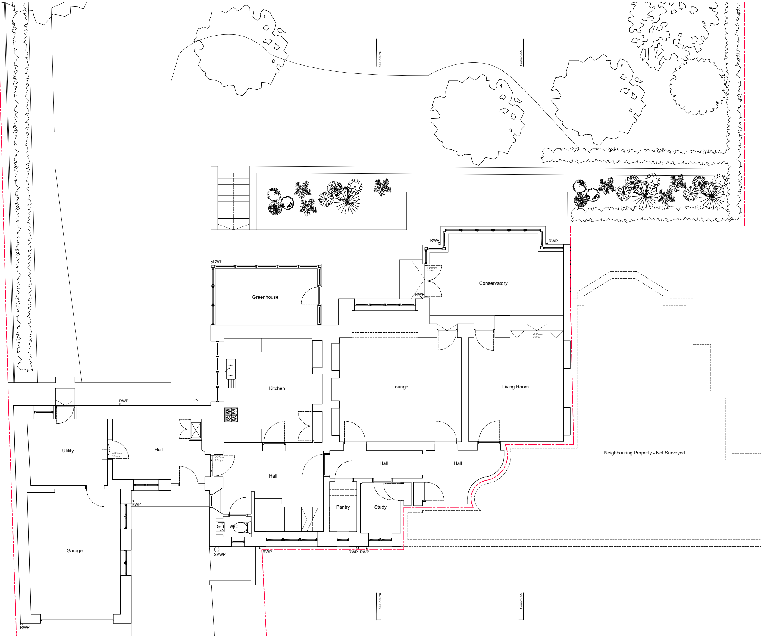
Ground Floor Plan as Existing @ 1:100
