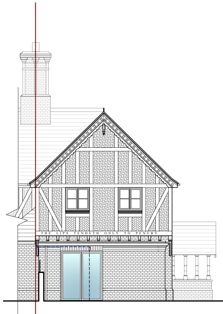
Proposed Rear Elevation (North West)
