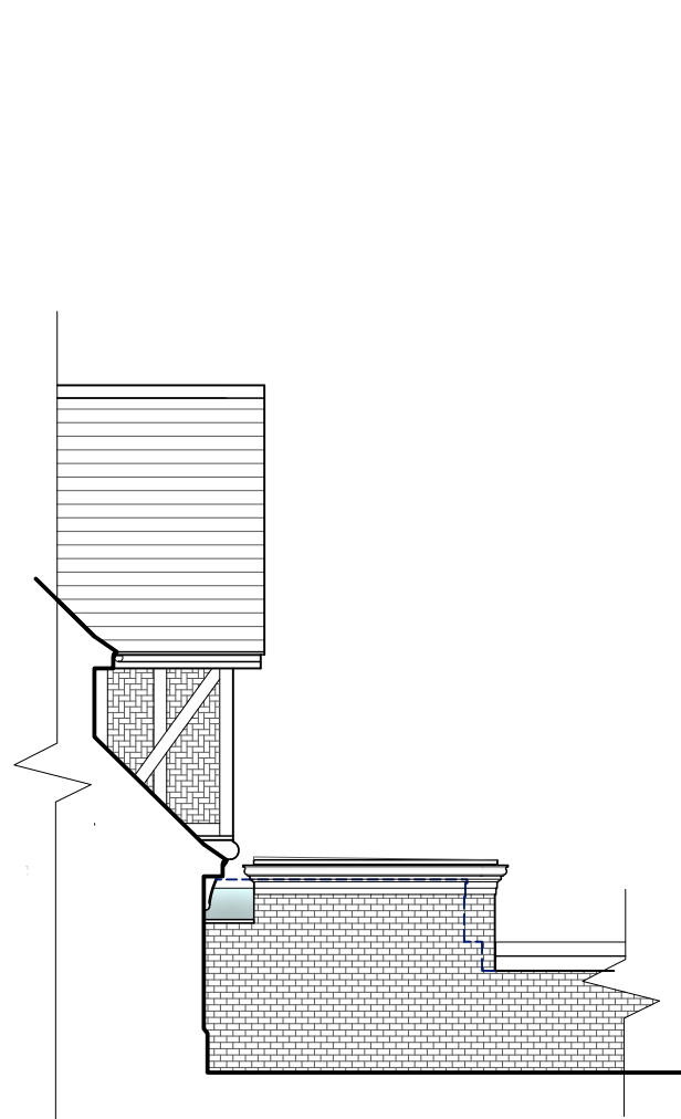
Proposed Side Elevation (North East)
