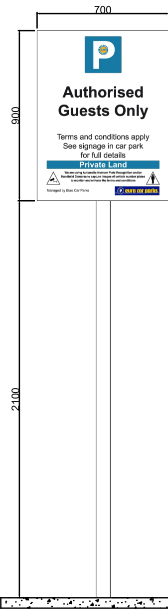
FRONT ELEVATION
