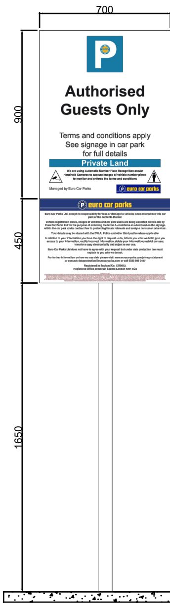
FRONT ELEVATION
