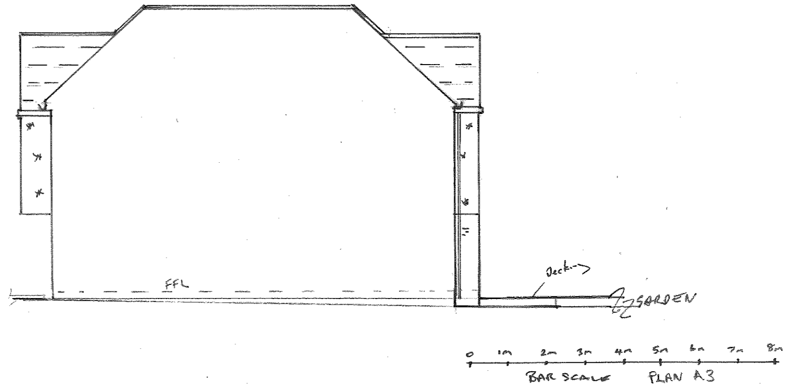
EXISTING SIDE ELEVATIONS
