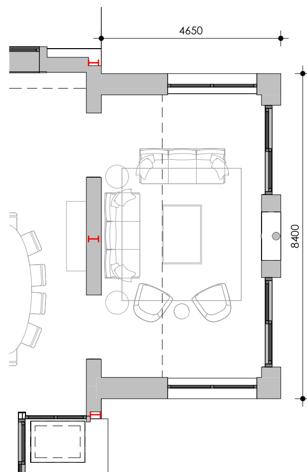
House 3 Extension_Ground floor FFL
