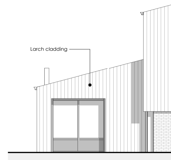
House 3 Extension_North elevation
