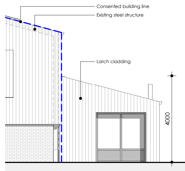
House 3 Extension_South elevation
