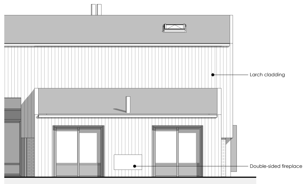
House 3 Extension_East elevation
