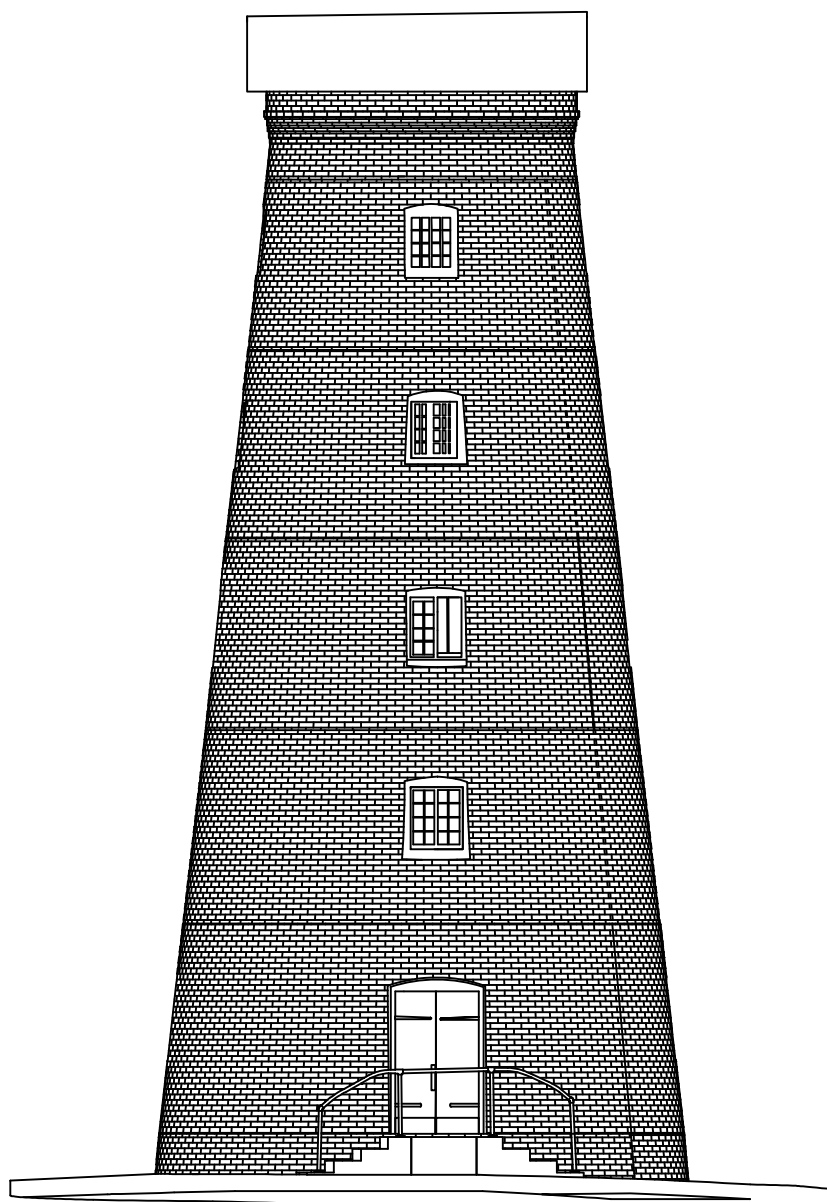
ELEVATION-01
