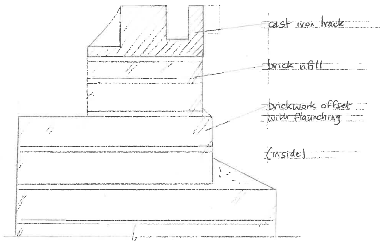
EXISTING BETWEEN CURB SECTION JOINTS
