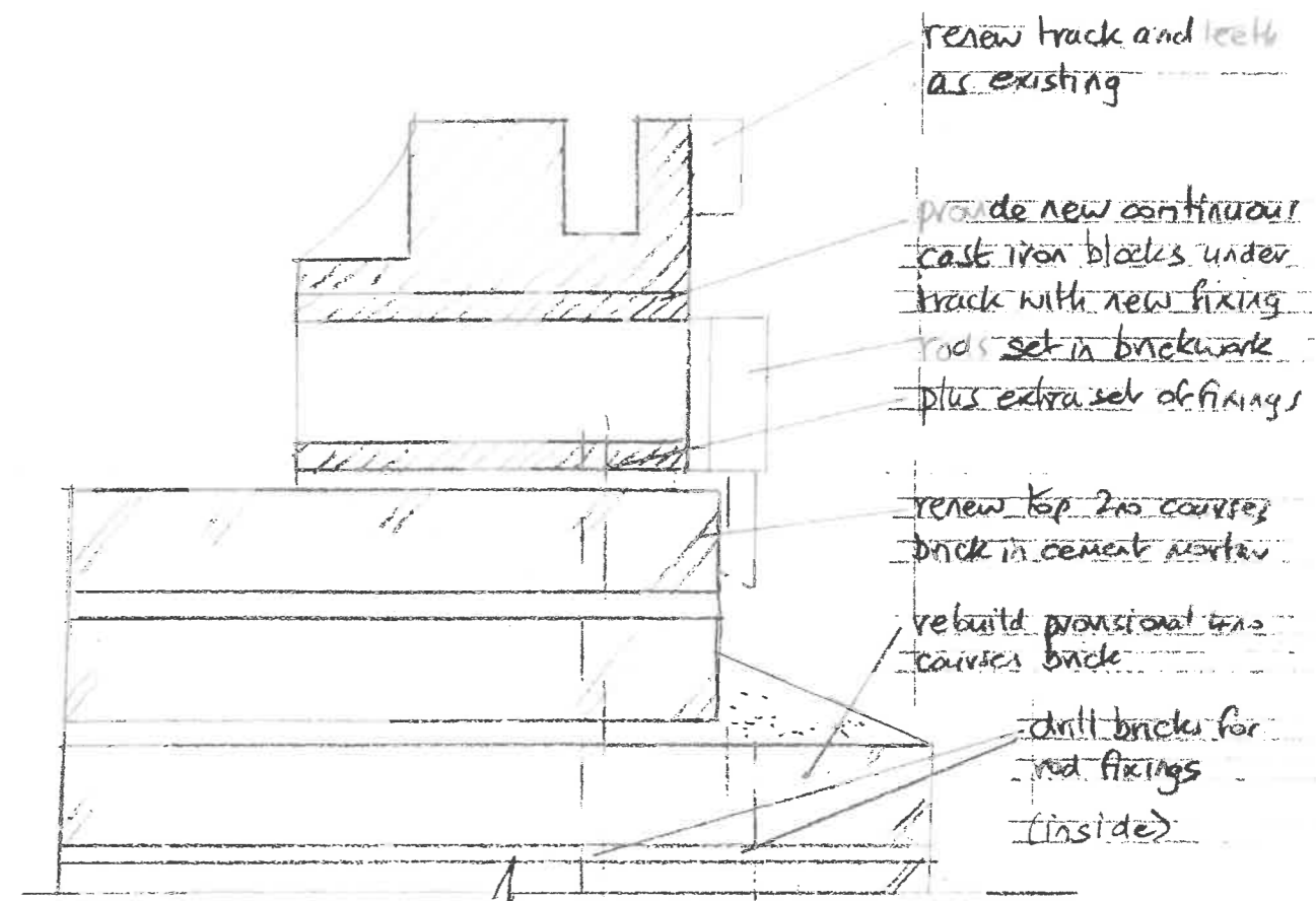
PROPOSED, GENERAL DETAIL SECTION
