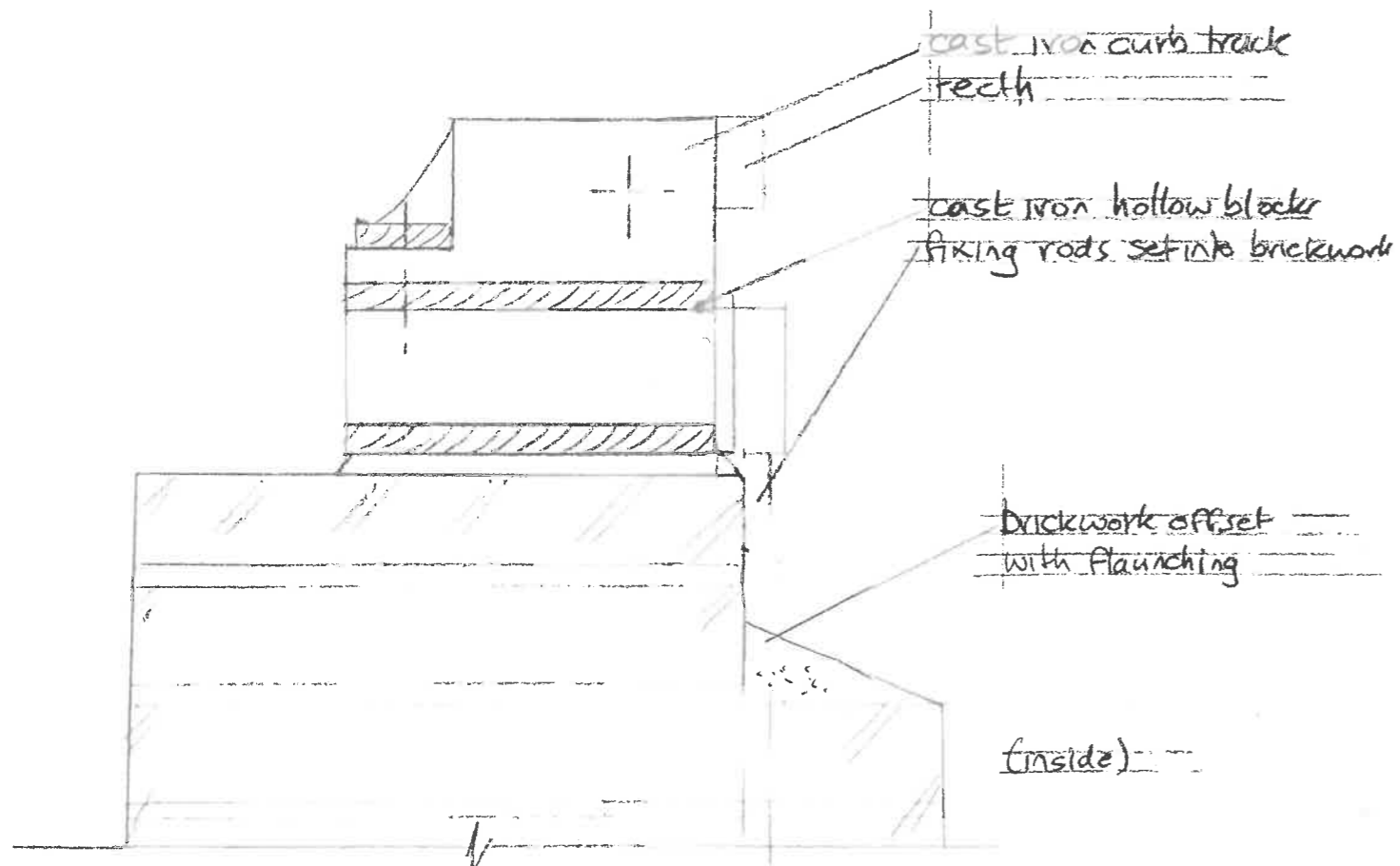
EXISTING AT CURB SECTION JOINTS
