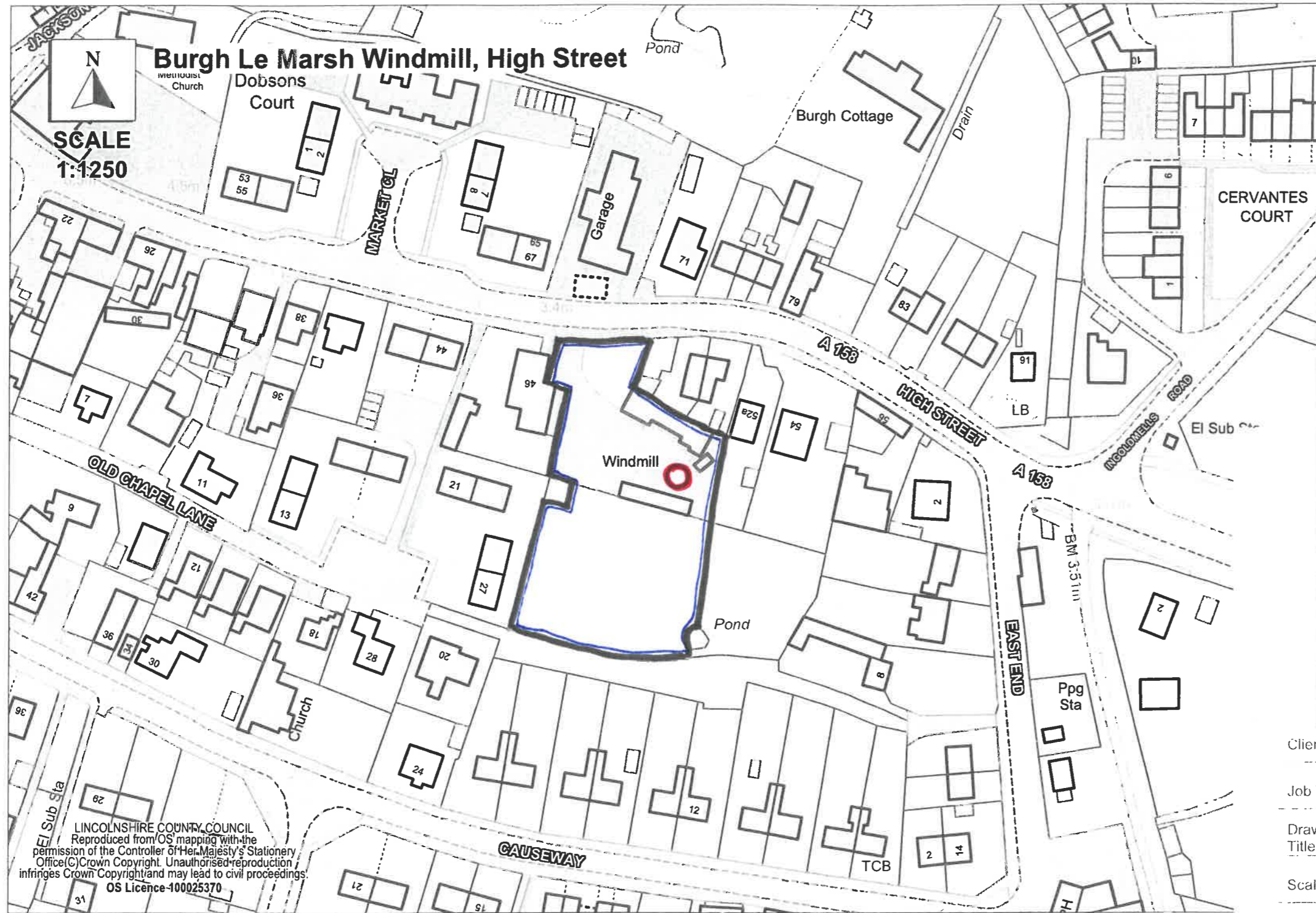
LOCATION PLAN @ 1:1250
