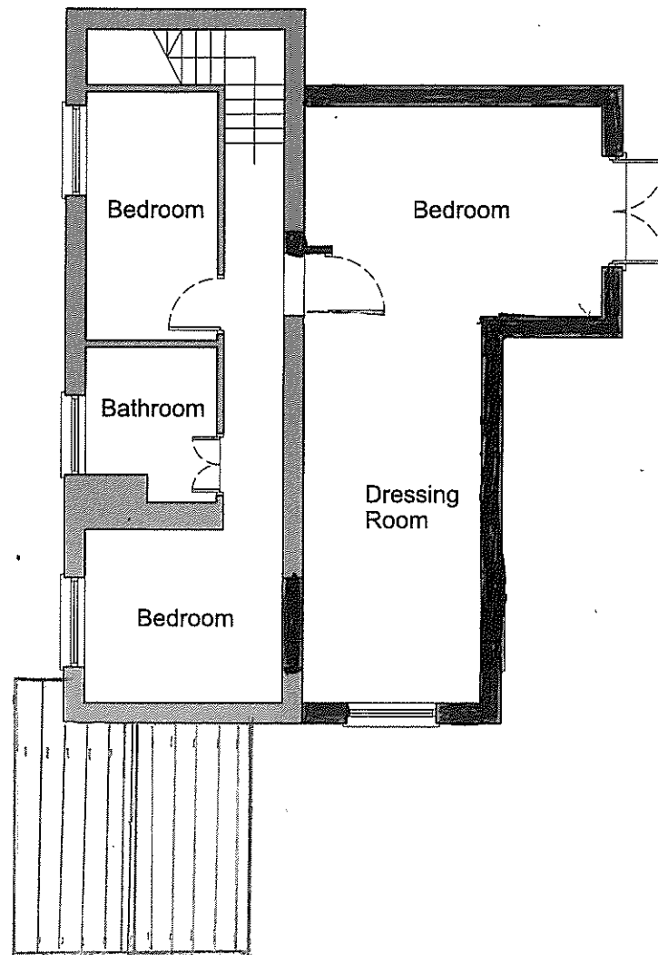
Proposed 1st Floor Plan
