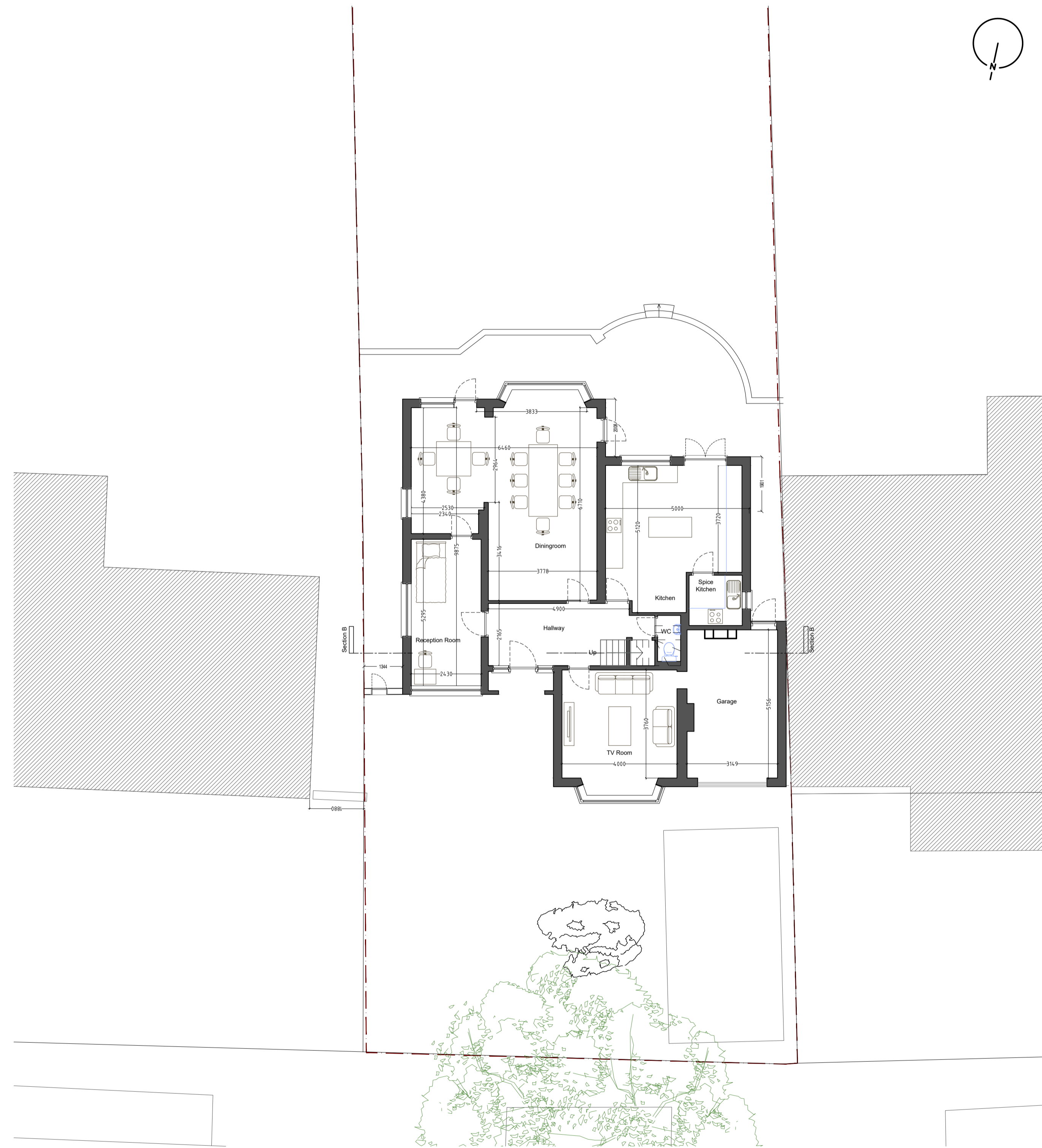
scale 1:100 0m 1m 2m 3m 4m 5m Ground Floor Plan - Existing
